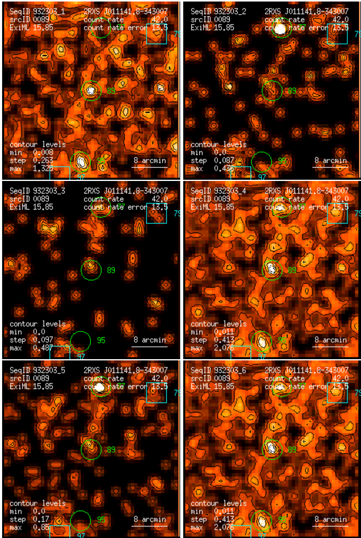
Figure 89: RASS 932303: detection 0089: band rate images, Gaussian filter: (1) PSPC channels 11 – 41, (2) 52 – 90, (3) 91 – 201, (4) 11 – 235, (5) 52 – 201, (6) 11 – 201. Broad band rates in counts/ks. Band rate contour levels in counts/ks/arcmin 2 .
