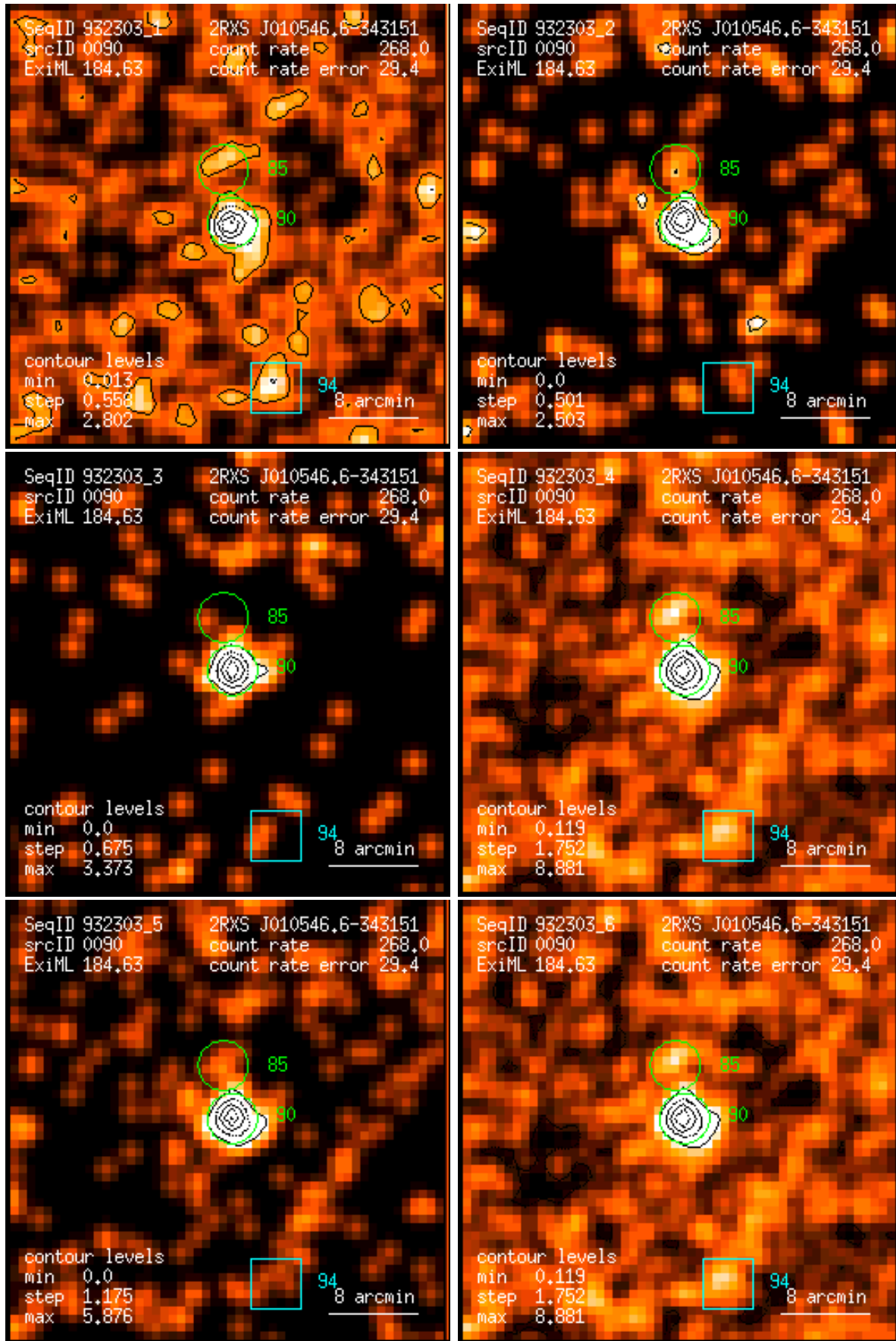
Figure 90: RASS 932303: detection 0090: band rate images, Gaussian filter: (1) PSPC channels 11 – 41, (2) 52 – 90, (3) 91 – 201, (4) 11 – 235, (5) 52 – 201, (6) 11 – 201. Broad band rates in counts/ks. Band rate contour levels in counts/ks/arcmin 2 .
