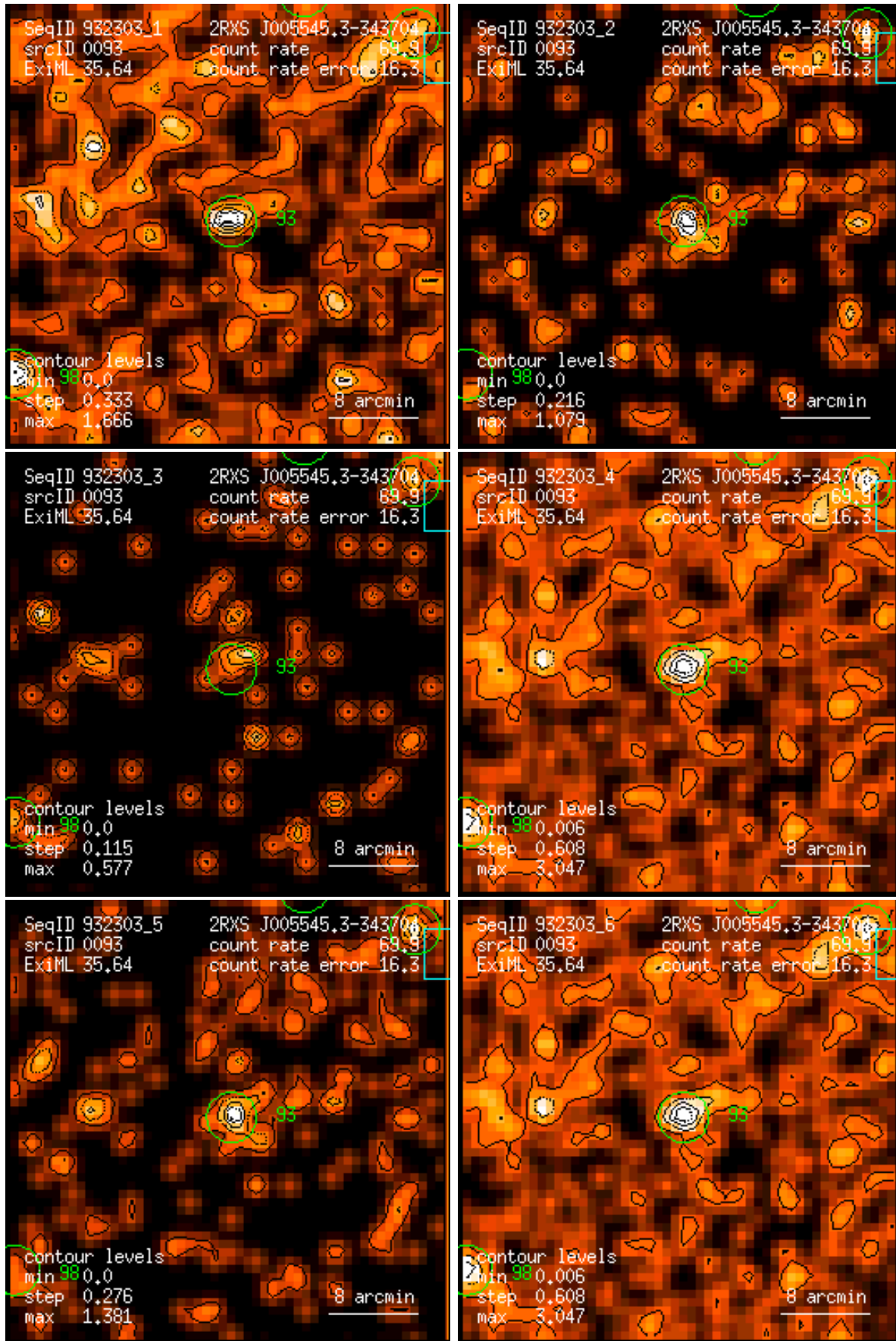
Figure 93: RASS 932303: detection 0093: band rate images, Gaussian filter: (1) PSPC channels 11 – 41, (2) 52 – 90, (3) 91 – 201, (4) 11 – 235, (5) 52 – 201, (6) 11 – 201. Broad band rates in counts/ks. Band rate contour levels in counts/ks/arcmin 2 .
