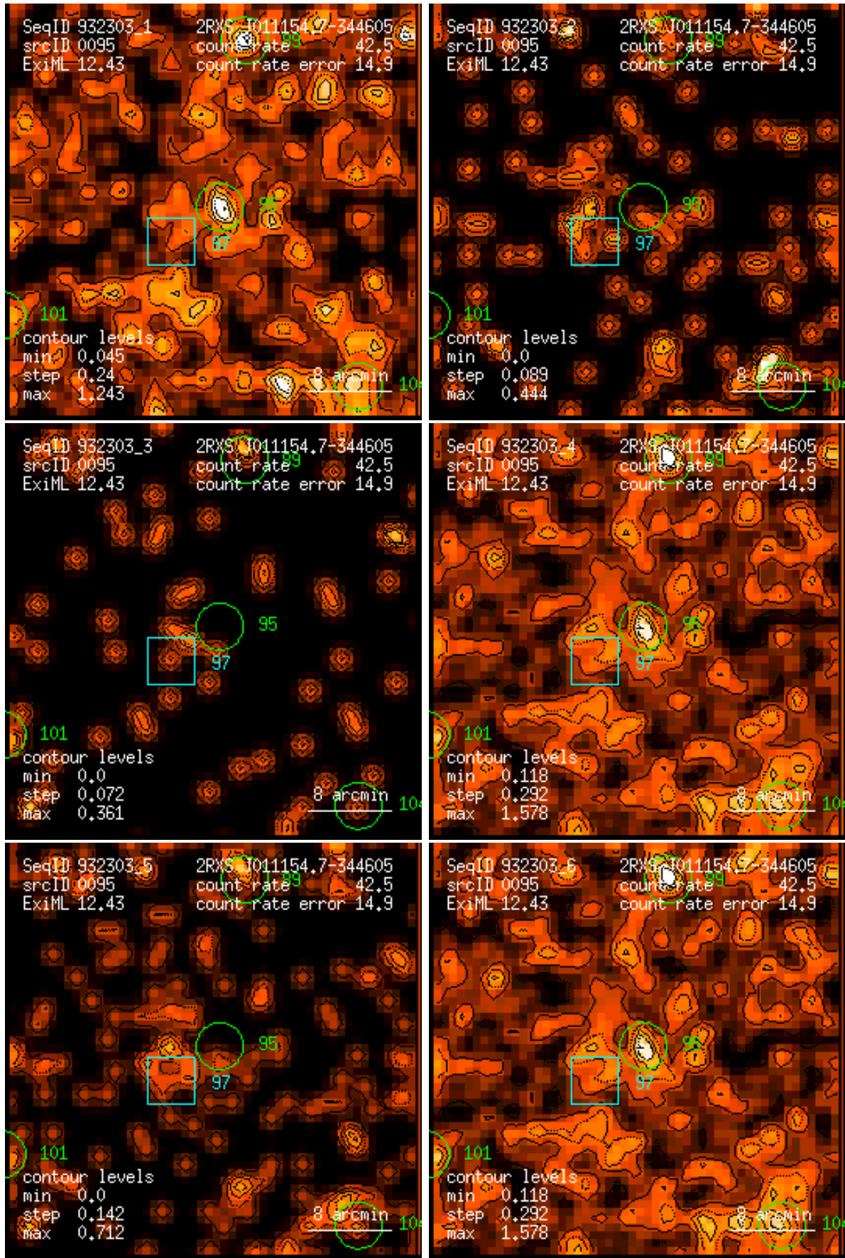
Figure 95: RASS 932303: detection 0095: band rate images, Gaussian filter: (1) PSPC channels 11 – 41, (2) 52 – 90, (3) 91 – 201, (4) 11 – 235, (5) 52 – 201, (6) 11 – 201. Broad band rates in counts/ks. Band rate contour levels in counts/ks/arcmin 2 .
