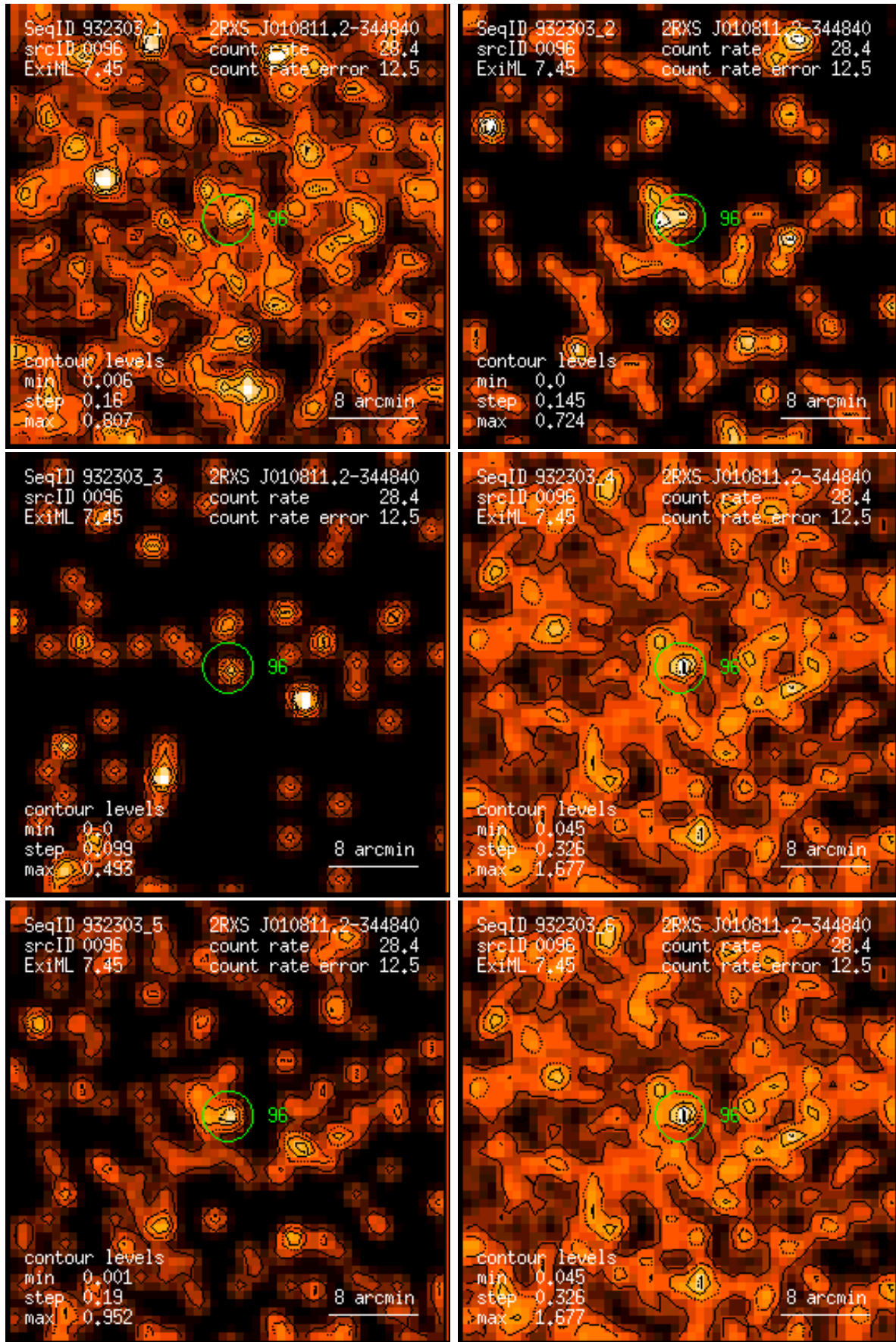
Figure 96: RASS 932303: detection 0096: band rate images, Gaussian filter: (1) PSPC channels 11 – 41, (2) 52 – 90, (3) 91 – 201, (4) 11 – 235, (5) 52 – 201, (6) 11 – 201. Broad band rates in counts/ks. Band rate contour levels in counts/ks/arcmin 2 .
