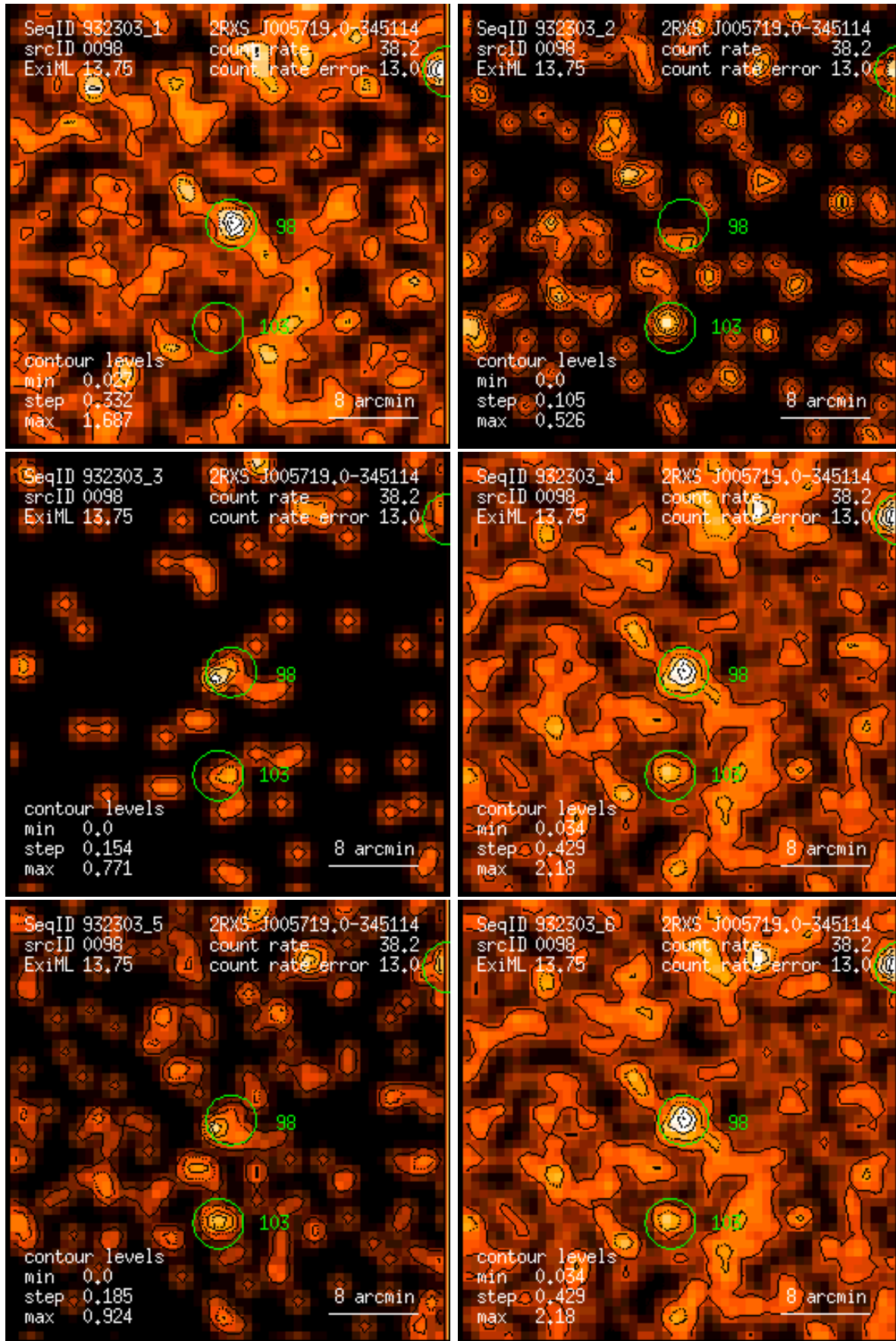
Figure 98: RASS 932303: detection 0098: band rate images, Gaussian filter: (1) PSPC channels 11 – 41, (2) 52 – 90, (3) 91 – 201, (4) 11 – 235, (5) 52 – 201, (6) 11 – 201. Broad band rates in counts/ks. Band rate contour levels in counts/ks/arcmin 2 .
