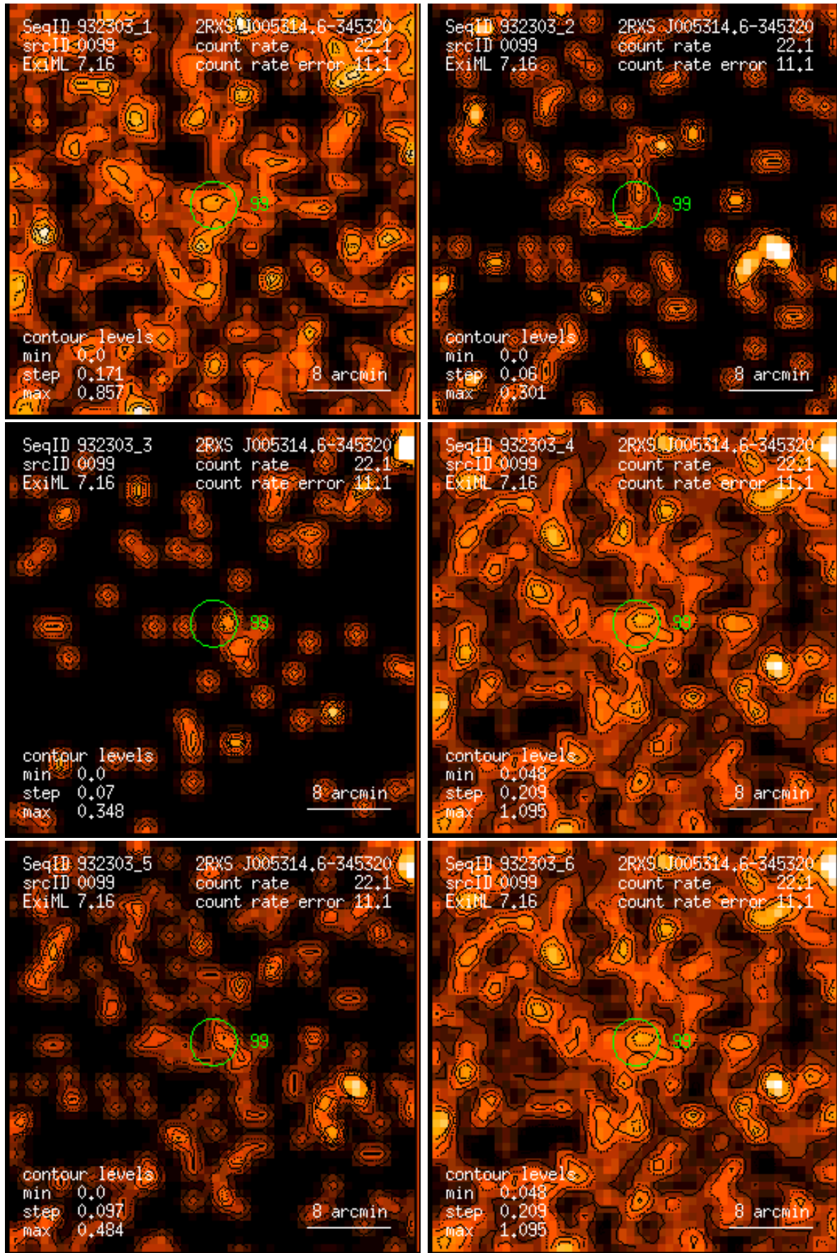
Figure 99: RASS 932303: detection 0099: band rate images, Gaussian filter: (1) PSPC channels 11 – 41, (2) 52 – 90, (3) 91 – 201, (4) 11 – 235, (5) 52 – 201, (6) 11 – 201. Broad band rates in counts/ks. Band rate contour levels in counts/ks/arcmin 2 .
