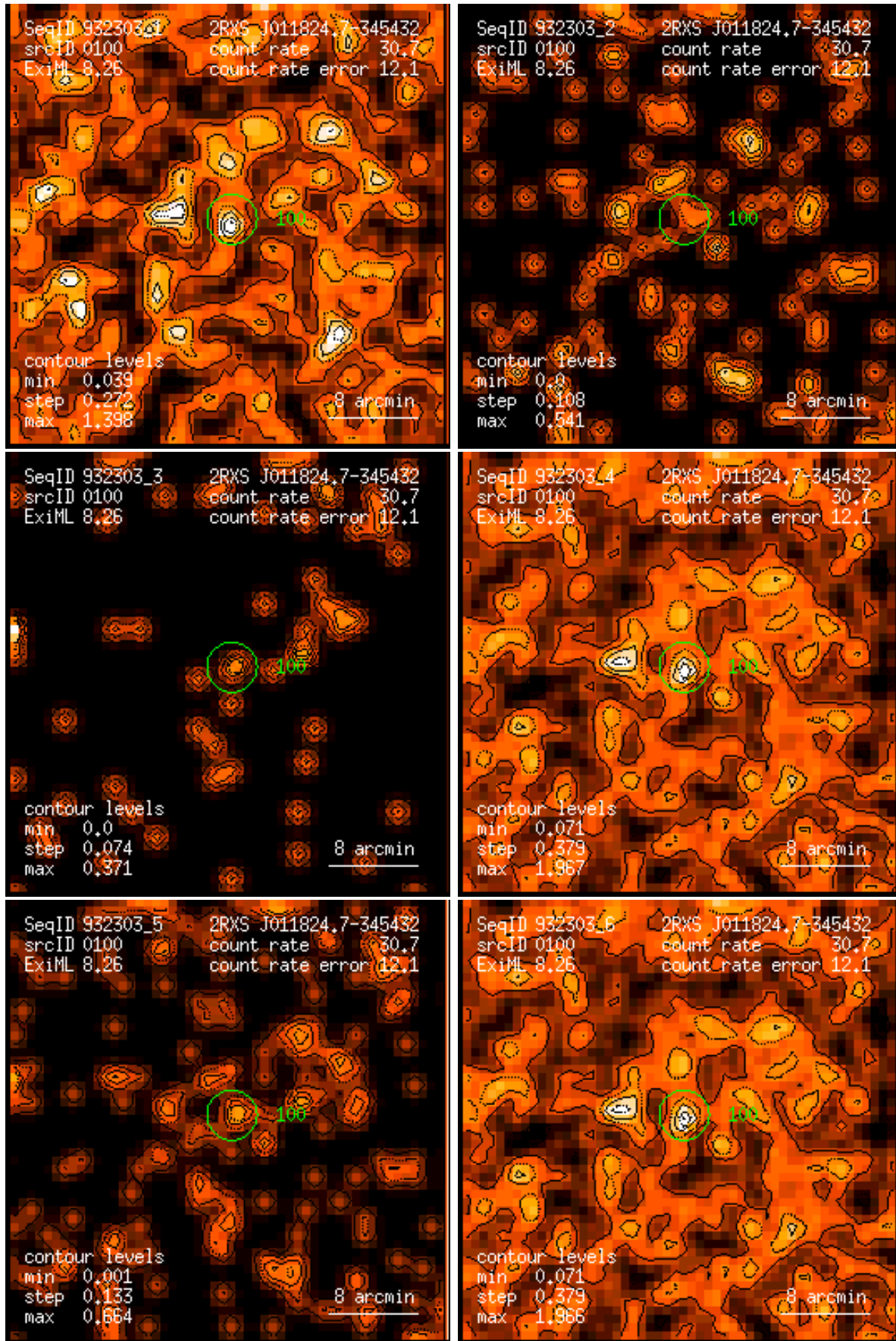
Figure 100: RASS 932303: detection 0100: band rate images, Gaussian filter: (1) PSPC channels 11 – 41, (2) 52 – 90, (3) 91 – 201, (4) 11 – 235, (5) 52 – 201, (6) 11 – 201. Broad band rates in counts/ks. Band rate contour levels in counts/ks/arcmin 2 .
