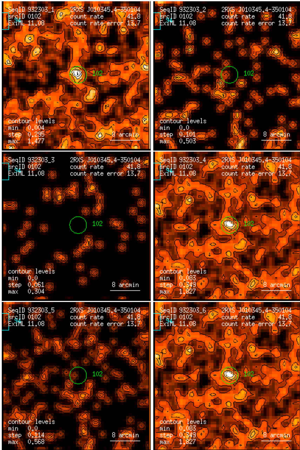
Figure 102: RASS 932303: detection 0102: band rate images, Gaussian filter: (1) PSPC channels 11 – 41, (2) 52 – 90, (3) 91 – 201, (4) 11 – 235, (5) 52 – 201, (6) 11 – 201. Broad band rates in counts/ks. Band rate contour levels in counts/ks/arcmin 2 .
