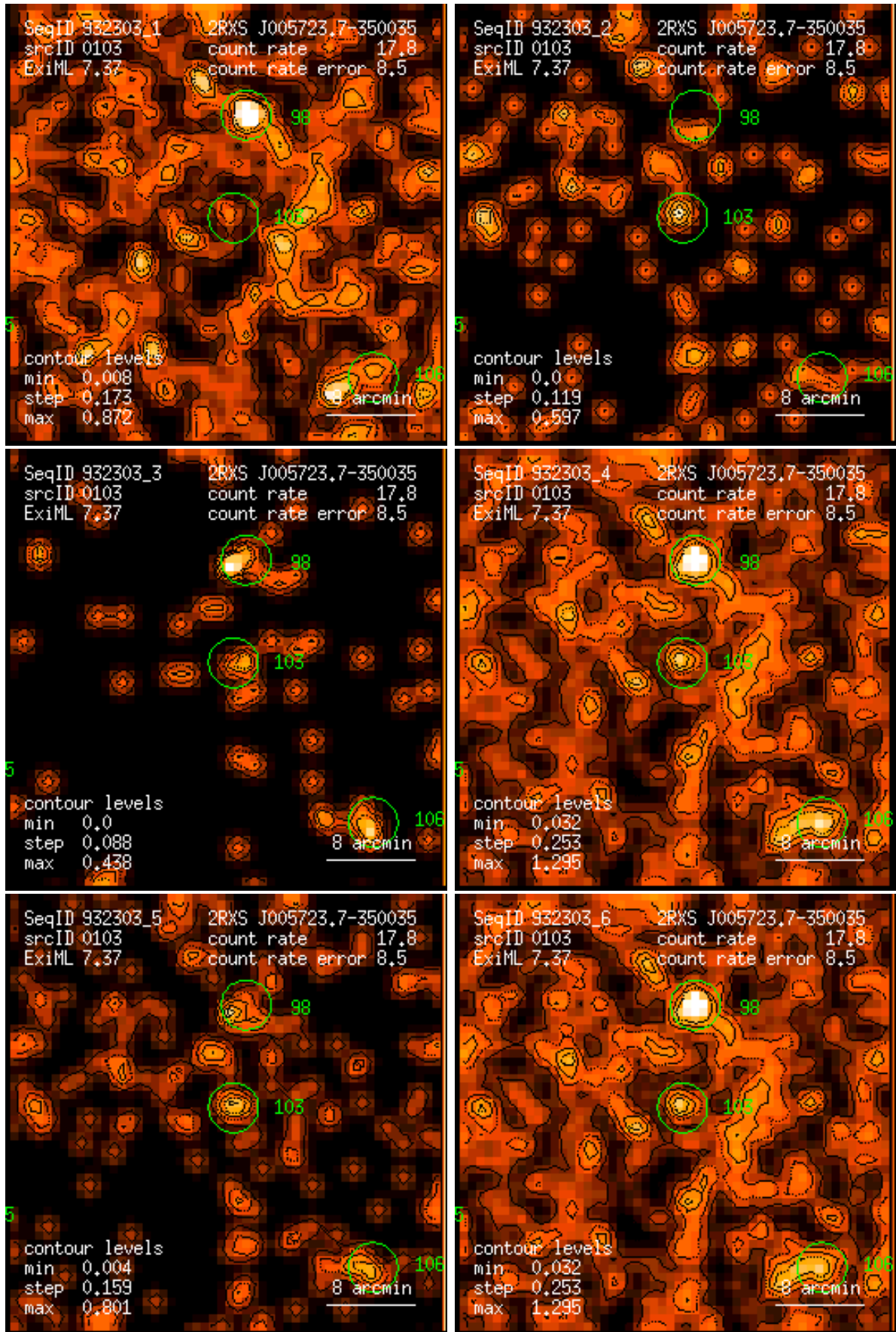
Figure 103: RASS 932303: detection 0103: band rate images, Gaussian filter: (1) PSPC channels 11 – 41, (2) 52 – 90, (3) 91 – 201, (4) 11 – 235, (5) 52 – 201, (6) 11 – 201. Broad band rates in counts/ks. Band rate contour levels in counts/ks/arcmin 2 .
