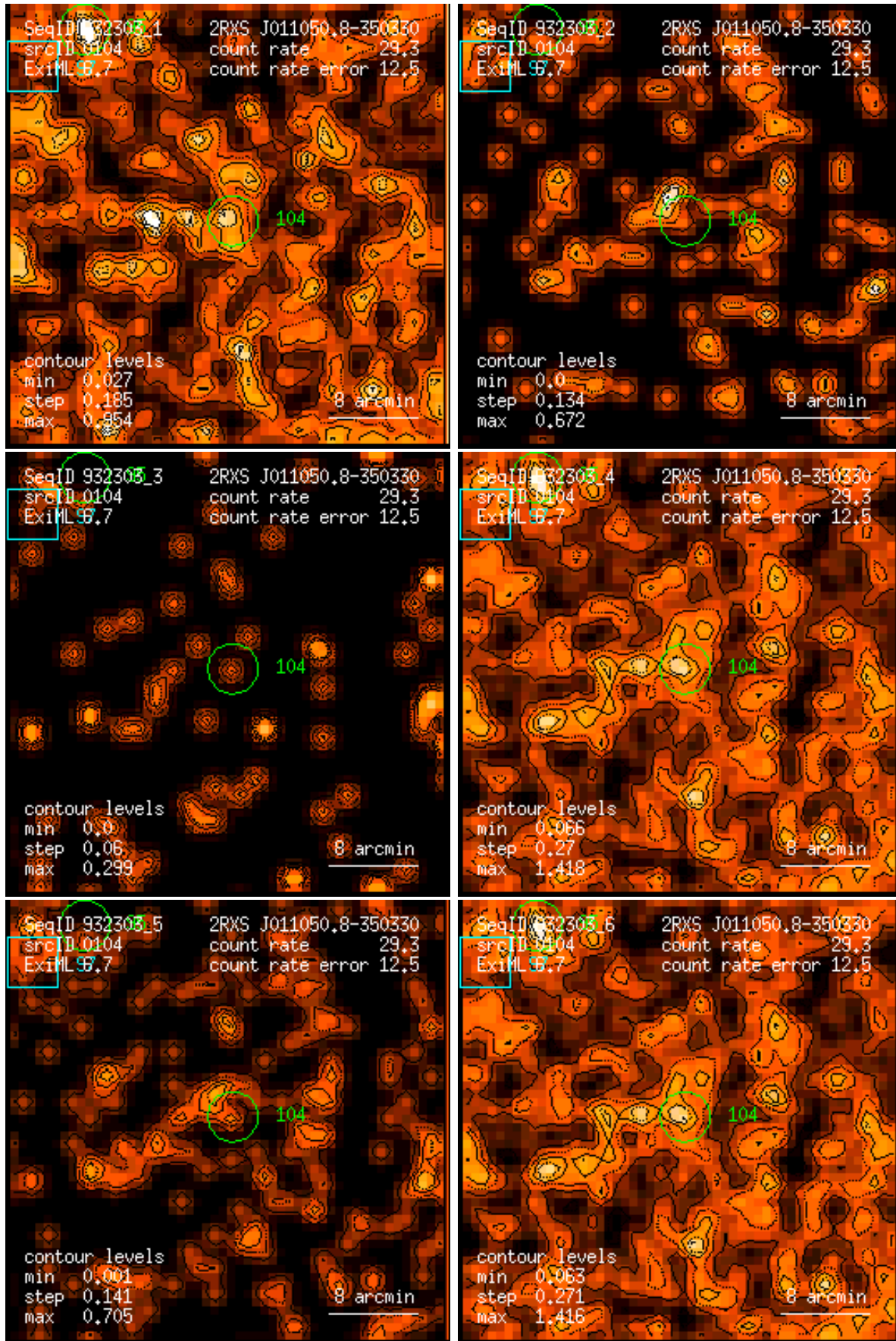
Figure 104: RASS 932303: detection 0104: band rate images, Gaussian filter: (1) PSPC channels 11 – 41, (2) 52 – 90, (3) 91 – 201, (4) 11 – 235, (5) 52 – 201, (6) 11 – 201. Broad band rates in counts/ks. Band rate contour levels in counts/ks/arcmin 2 .
