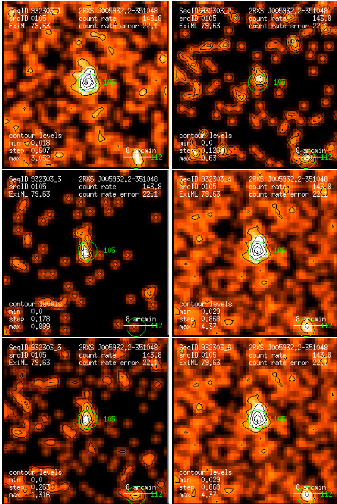
Figure 105: RASS 932303: detection 0105: band rate images, Gaussian filter: (1) PSPC channels 11 – 41, (2) 52 – 90, (3) 91 – 201, (4) 11 – 235, (5) 52 – 201, (6) 11 – 201. Broad band rates in counts/ks. Band rate contour levels in counts/ks/arcmin 2 .
