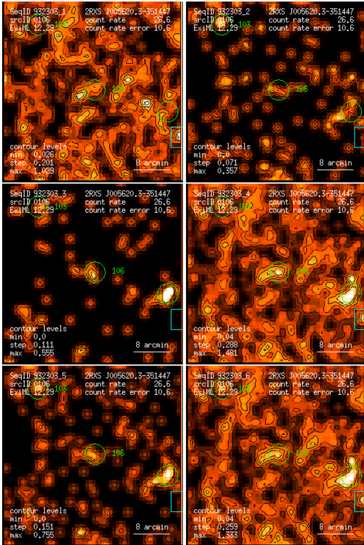
Figure 106: RASS 932303: detection 0106: band rate images, Gaussian filter: (1) PSPC channels 11 – 41, (2) 52 – 90, (3) 91 – 201, (4) 11 – 235, (5) 52 – 201, (6) 11 – 201. Broad band rates in counts/ks. Band rate contour levels in counts/ks/arcmin 2 .
