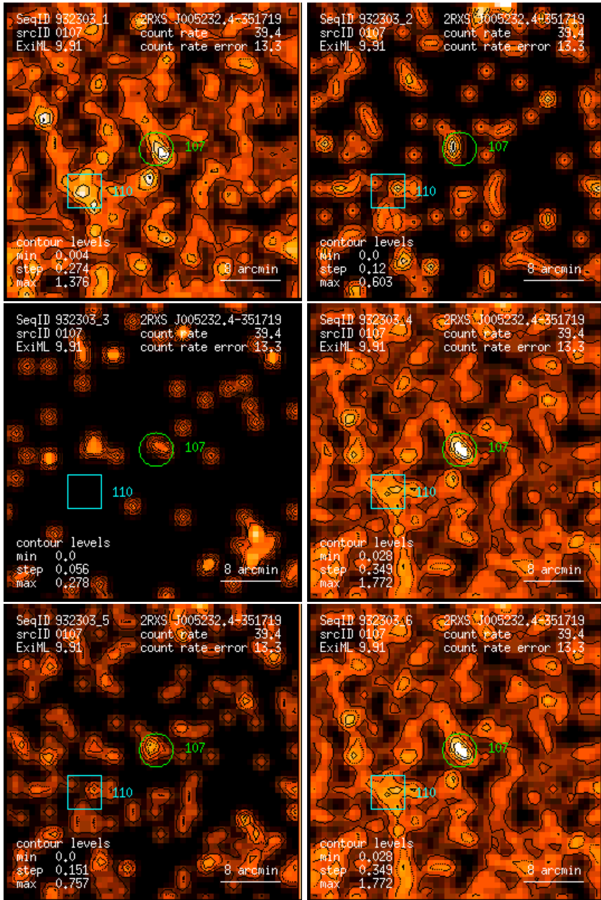
Figure 107: RASS 932303: detection 0107: band rate images, Gaussian filter: (1) PSPC channels 11 – 41, (2) 52 – 90, (3) 91 – 201, (4) 11 – 235, (5) 52 – 201, (6) 11 – 201. Broad band rates in counts/ks. Band rate contour levels in counts/ks/arcmin 2 .
