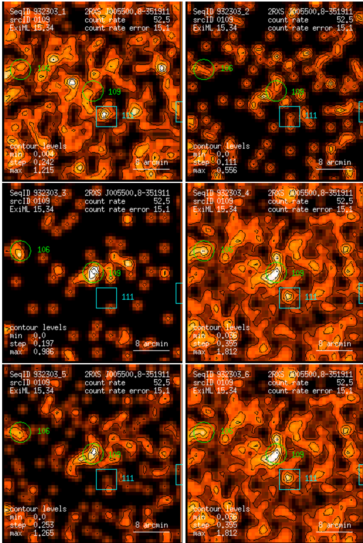
Figure 109: RASS 932303: detection 0109: band rate images, Gaussian filter: (1) PSPC channels 11 – 41, (2) 52 – 90, (3) 91 – 201, (4) 11 – 235, (5) 52 – 201, (6) 11 – 201. Broad band rates in counts/ks. Band rate contour levels in counts/ks/arcmin 2 .
