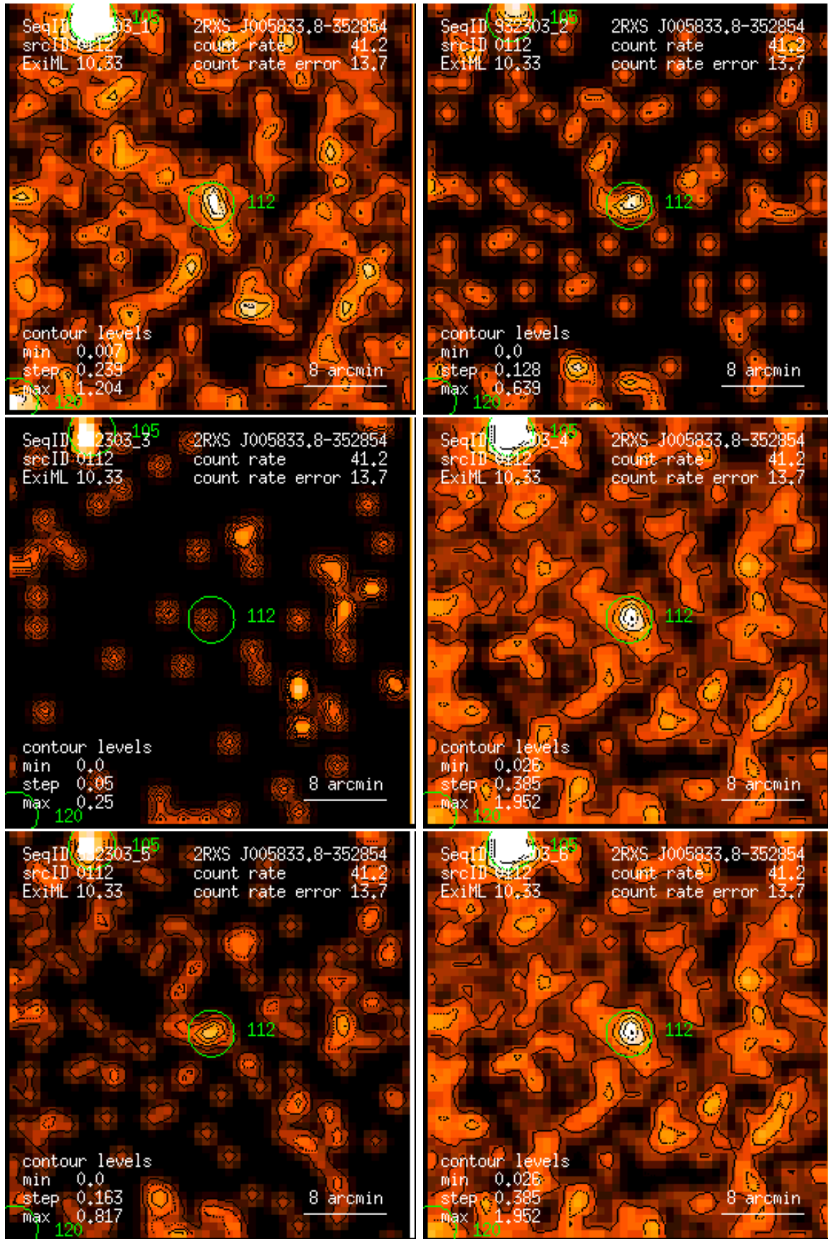
Figure 112: RASS 932303: detection 0112: band rate images, Gaussian filter: (1) PSPC channels 11 – 41, (2) 52 – 90, (3) 91 – 201, (4) 11 – 235, (5) 52 – 201, (6) 11 – 201. Broad band rates in counts/ks. Band rate contour levels in counts/ks/arcmin 2 .
