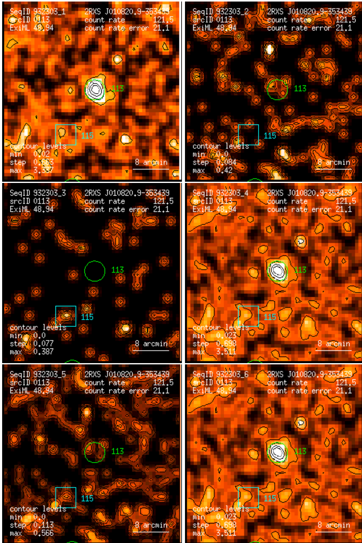
Figure 113: RASS 932303: detection 0113: band rate images, Gaussian filter: (1) PSPC channels 11 – 41, (2) 52 – 90, (3) 91 – 201, (4) 11 – 235, (5) 52 – 201, (6) 11 – 201. Broad band rates in counts/ks. Band rate contour levels in counts/ks/arcmin 2 .
