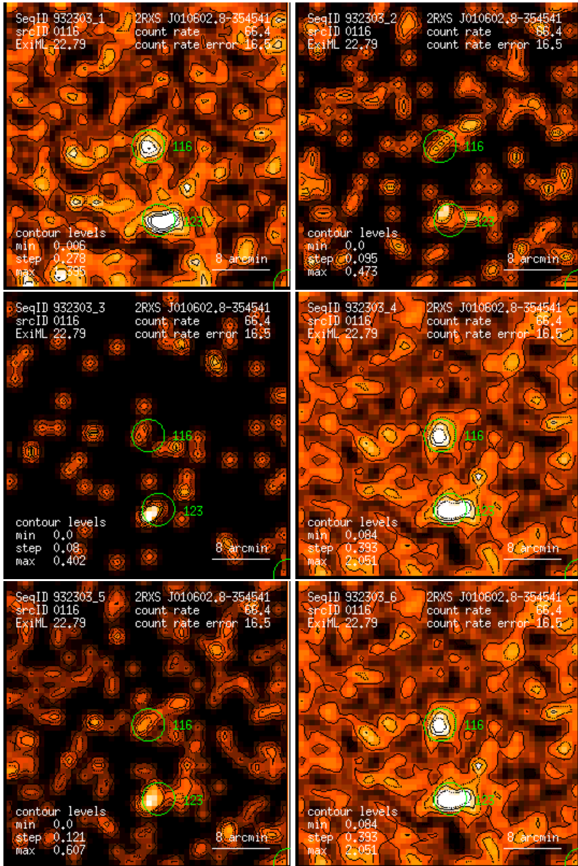
Figure 116: RASS 932303: detection 0116: band rate images, Gaussian filter: (1) PSPC channels 11 – 41, (2) 52 – 90, (3) 91 – 201, (4) 11 – 235, (5) 52 – 201, (6) 11 – 201. Broad band rates in counts/ks. Band rate contour levels in counts/ks/arcmin 2 .
