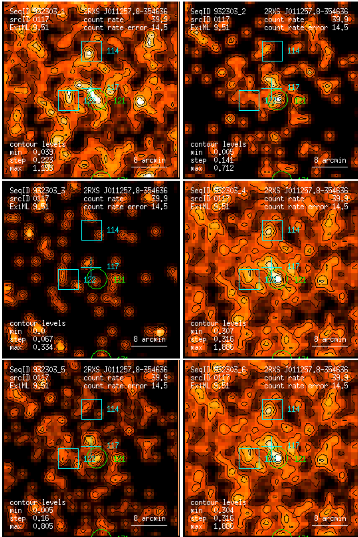
Figure 117: RASS 932303: detection 0117: band rate images, Gaussian filter: (1) PSPC channels 11 – 41, (2) 52 – 90, (3) 91 – 201, (4) 11 – 235, (5) 52 – 201, (6) 11 – 201. Broad band rates in counts/ks. Band rate contour levels in counts/ks/arcmin 2 .
