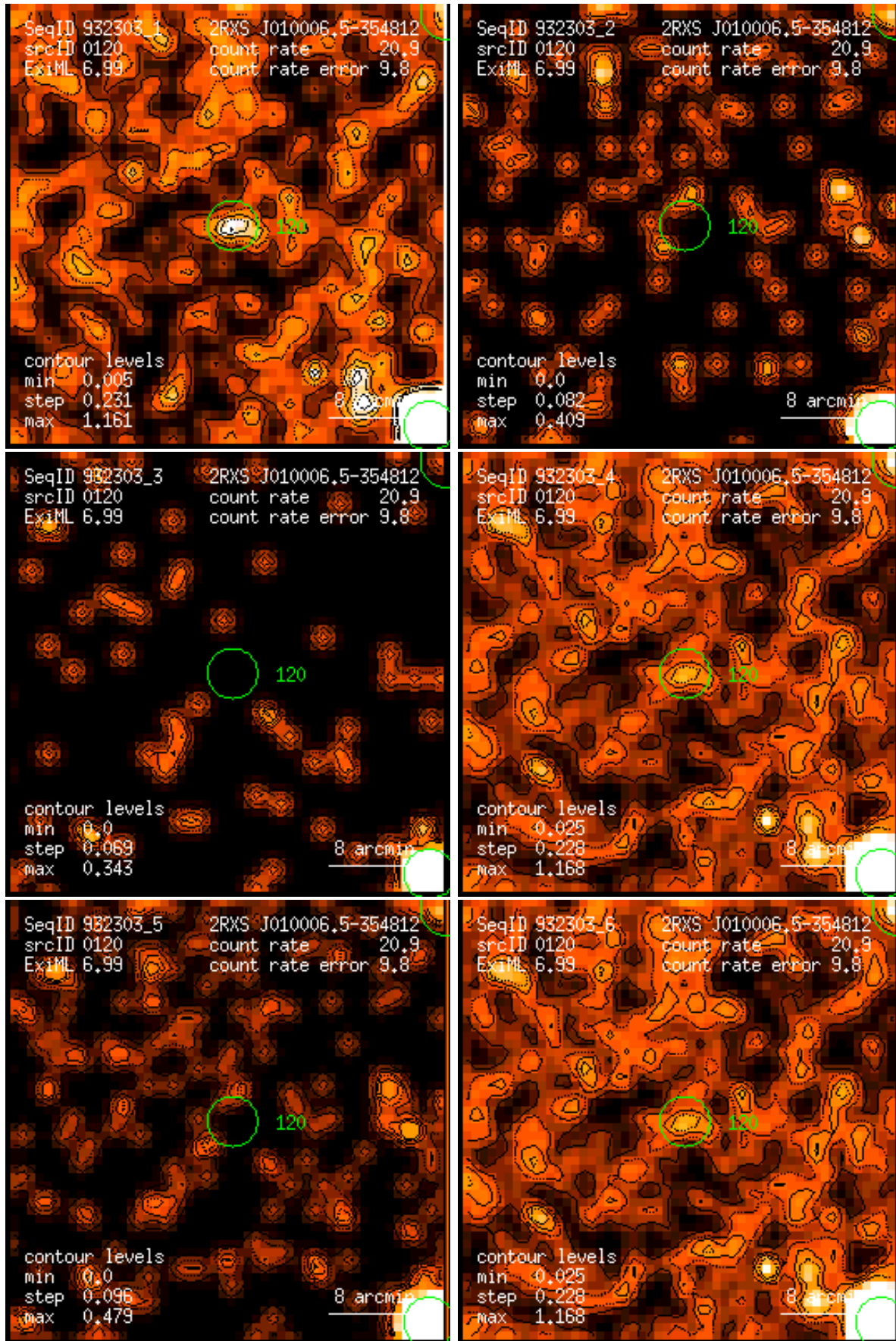
Figure 120: RASS 932303: detection 0120: band rate images, Gaussian filter: (1) PSPC channels 11 – 41, (2) 52 – 90, (3) 91 – 201, (4) 11 – 235, (5) 52 – 201, (6) 11 – 201. Broad band rates in counts/ks. Band rate contour levels in counts/ks/arcmin 2 .
