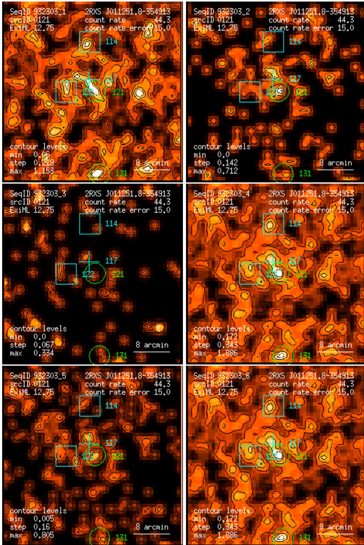
Figure 121: RASS 932303: detection 0121: band rate images, Gaussian filter: (1) PSPC channels 11 – 41, (2) 52 – 90, (3) 91 – 201, (4) 11 – 235, (5) 52 – 201, (6) 11 – 201. Broad band rates in counts/ks. Band rate contour levels in counts/ks/arcmin 2 .
