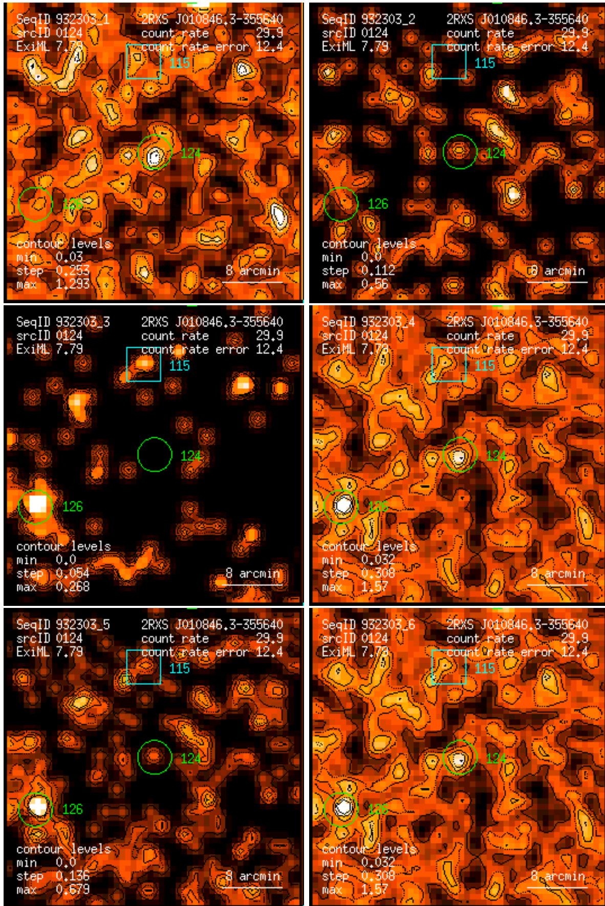
Figure 124: RASS 932303: detection 0124: band rate images, Gaussian filter: (1) PSPC channels 11 – 41, (2) 52 – 90, (3) 91 – 201, (4) 11 – 235, (5) 52 – 201, (6) 11 – 201. Broad band rates in counts/ks. Band rate contour levels in counts/ks/arcmin 2 .
