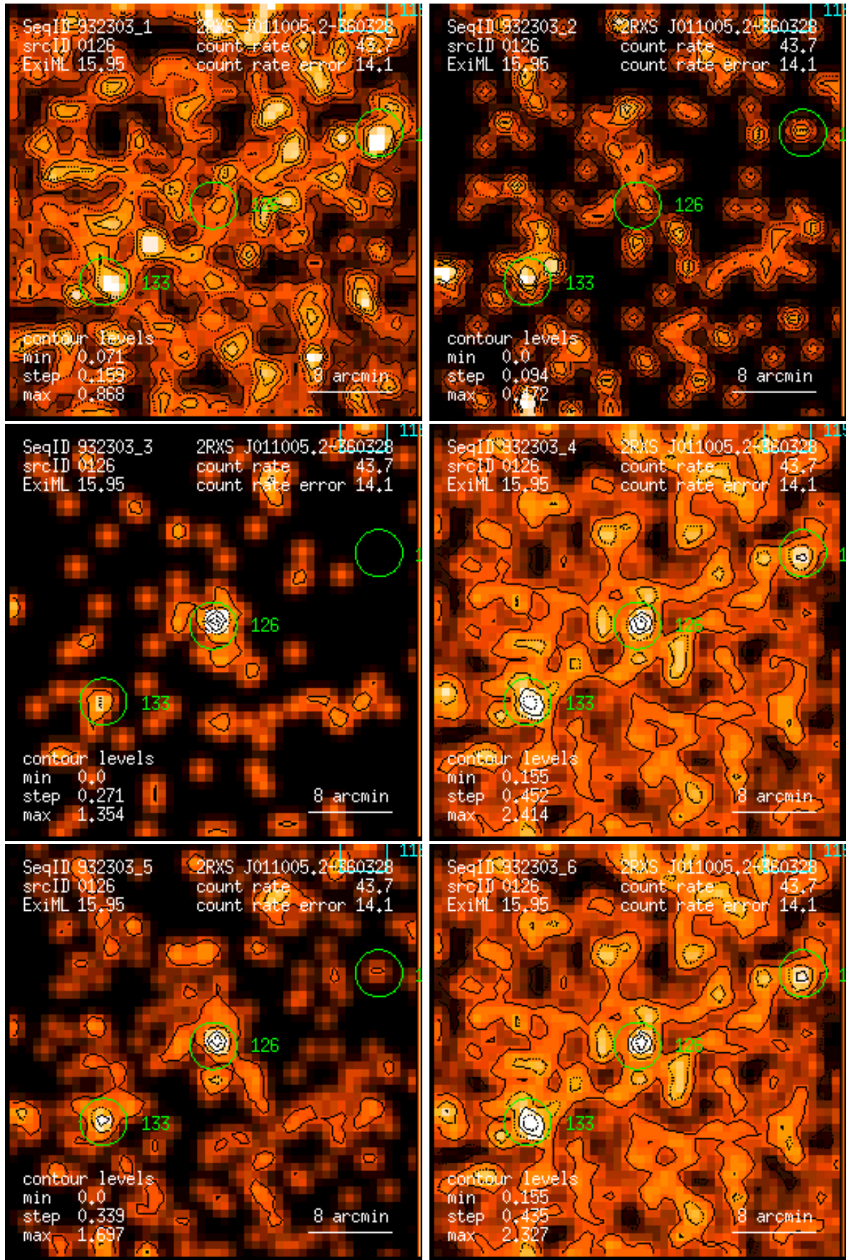
Figure 126: RASS 932303: detection 0126: band rate images, Gaussian filter: (1) PSPC channels 11 – 41, (2) 52 – 90, (3) 91 – 201, (4) 11 – 235, (5) 52 – 201, (6) 11 – 201. Broad band rates in counts/ks. Band rate contour levels in counts/ks/arcmin 2 .
