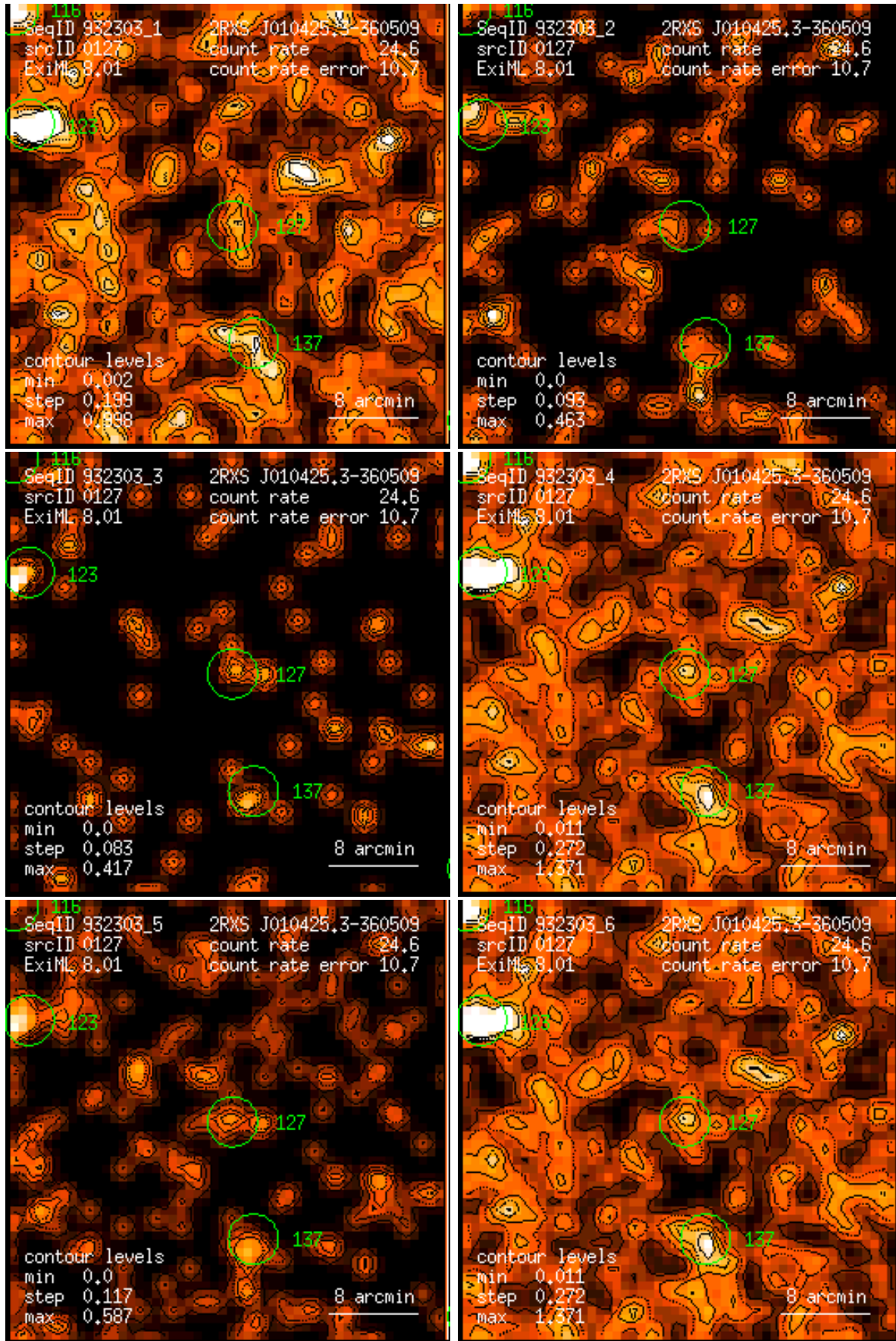
Figure 127: RASS 932303: detection 0127: band rate images, Gaussian filter: (1) PSPC channels 11 – 41, (2) 52 – 90, (3) 91 – 201, (4) 11 – 235, (5) 52 – 201, (6) 11 – 201. Broad band rates in counts/ks. Band rate contour levels in counts/ks/arcmin 2 .
