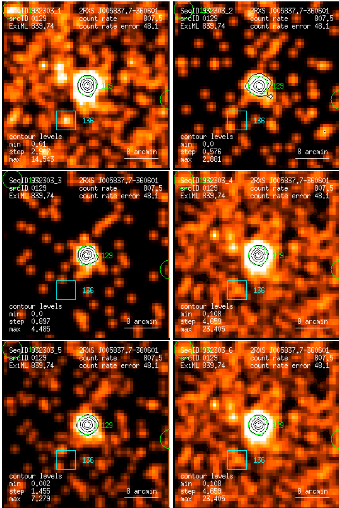
Figure 129: RASS 932303: detection 0129: band rate images, Gaussian filter: (1) PSPC channels 11 – 41, (2) 52 – 90, (3) 91 – 201, (4) 11 – 235, (5) 52 – 201, (6) 11 – 201. Broad band rates in counts/ks. Band rate contour levels in counts/ks/arcmin 2 .
