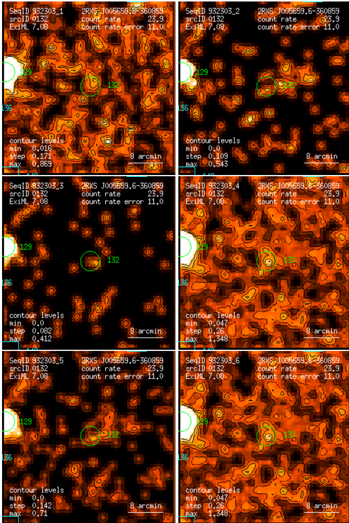
Figure 132: RASS 932303: detection 0132: band rate images, Gaussian filter: (1) PSPC channels 11 – 41, (2) 52 – 90, (3) 91 – 201, (4) 11 – 235, (5) 52 – 201, (6) 11 – 201. Broad band rates in counts/ks. Band rate contour levels in counts/ks/arcmin 2 .
