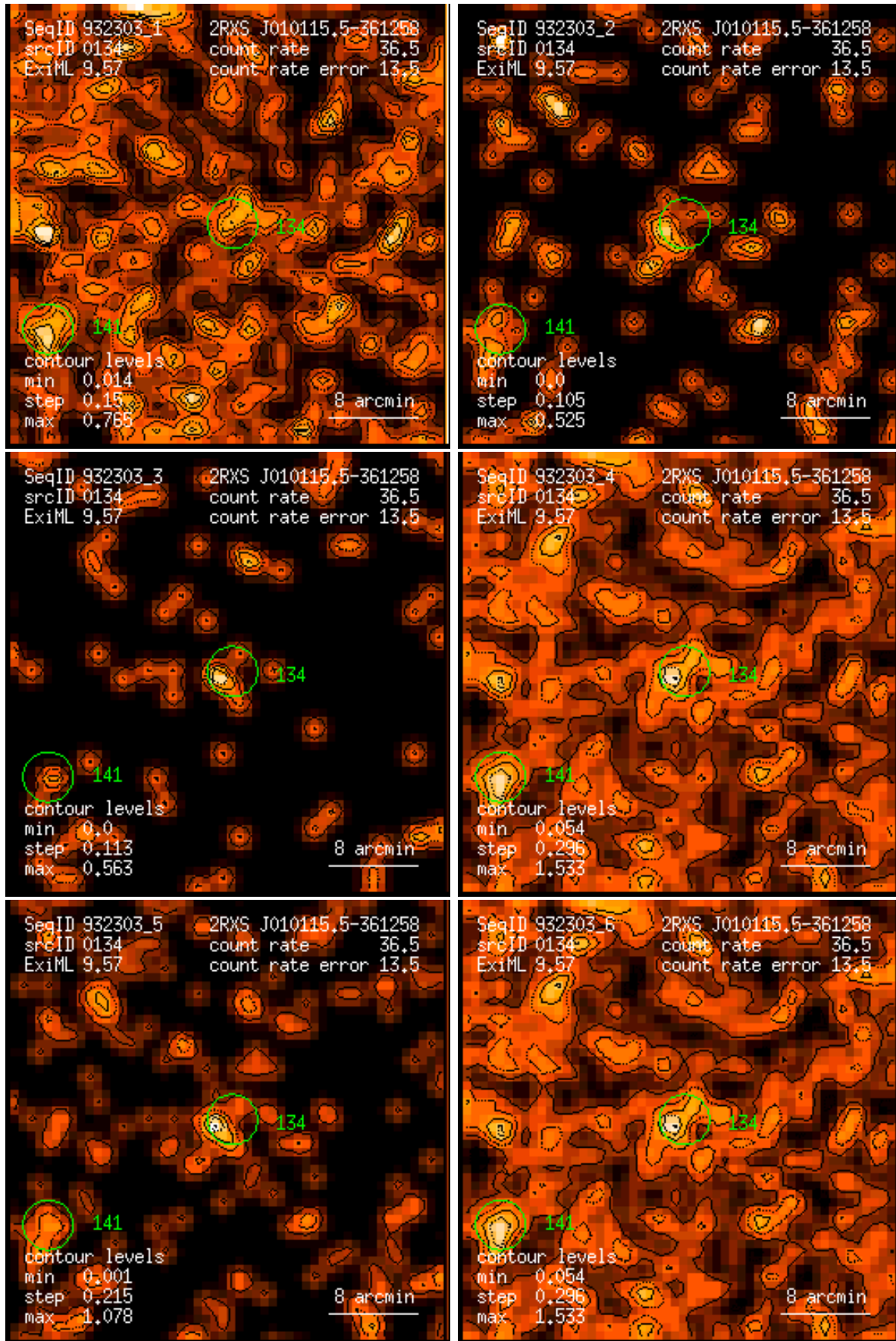
Figure 134: RASS 932303: detection 0134: band rate images, Gaussian filter: (1) PSPC channels 11 – 41, (2) 52 – 90, (3) 91 – 201, (4) 11 – 235, (5) 52 – 201, (6) 11 – 201. Broad band rates in counts/ks. Band rate contour levels in counts/ks/arcmin 2 .
