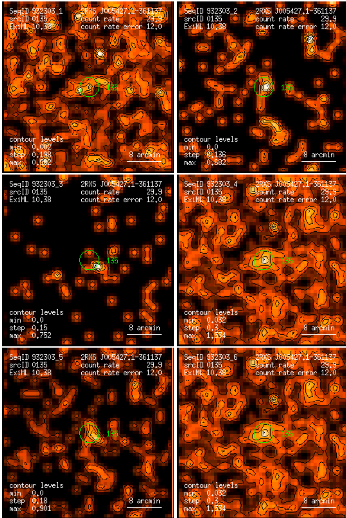
Figure 135: RASS 932303: detection 0135: band rate images, Gaussian filter: (1) PSPC channels 11 – 41, (2) 52 – 90, (3) 91 – 201, (4) 11 – 235, (5) 52 – 201, (6) 11 – 201. Broad band rates in counts/ks. Band rate contour levels in counts/ks/arcmin 2 .
