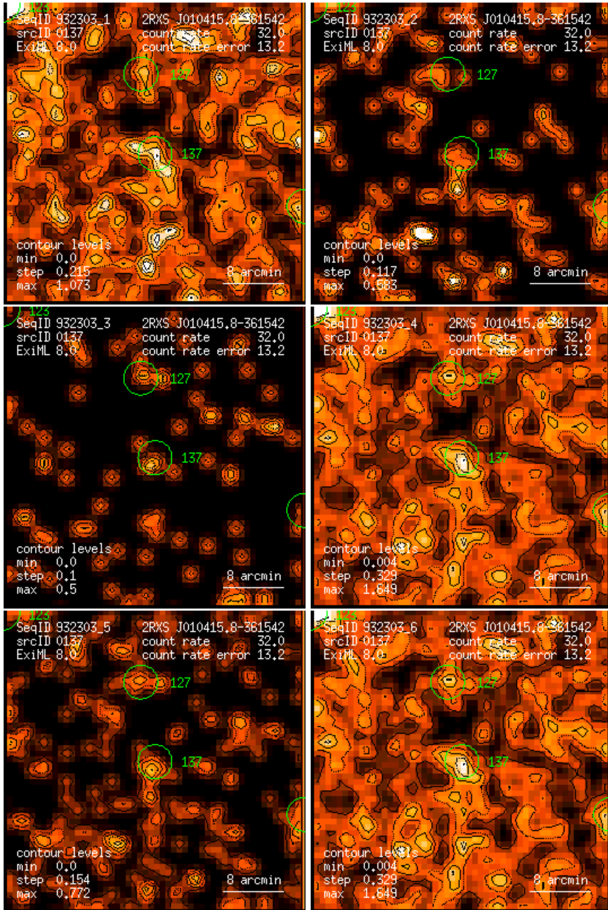
Figure 137: RASS 932303: detection 0137: band rate images, Gaussian filter: (1) PSPC channels 11 – 41, (2) 52 – 90, (3) 91 – 201, (4) 11 – 235, (5) 52 – 201, (6) 11 – 201. Broad band rates in counts/ks. Band rate contour levels in counts/ks/arcmin 2 .
