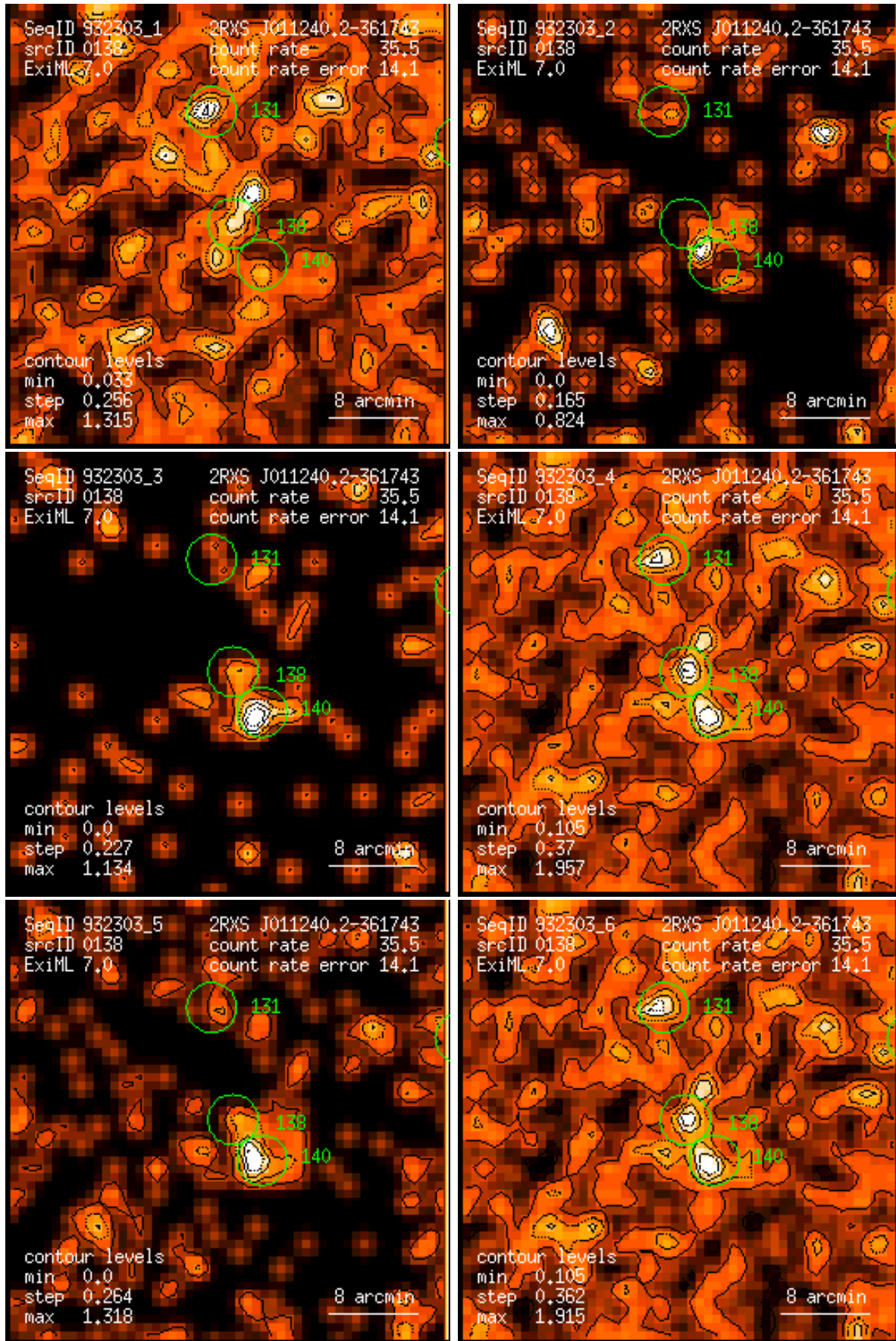
Figure 138: RASS 932303: detection 0138: band rate images, Gaussian filter: (1) PSPC channels 11 – 41, (2) 52 – 90, (3) 91 – 201, (4) 11 – 235, (5) 52 – 201, (6) 11 – 201. Broad band rates in counts/ks. Band rate contour levels in counts/ks/arcmin 2 .
