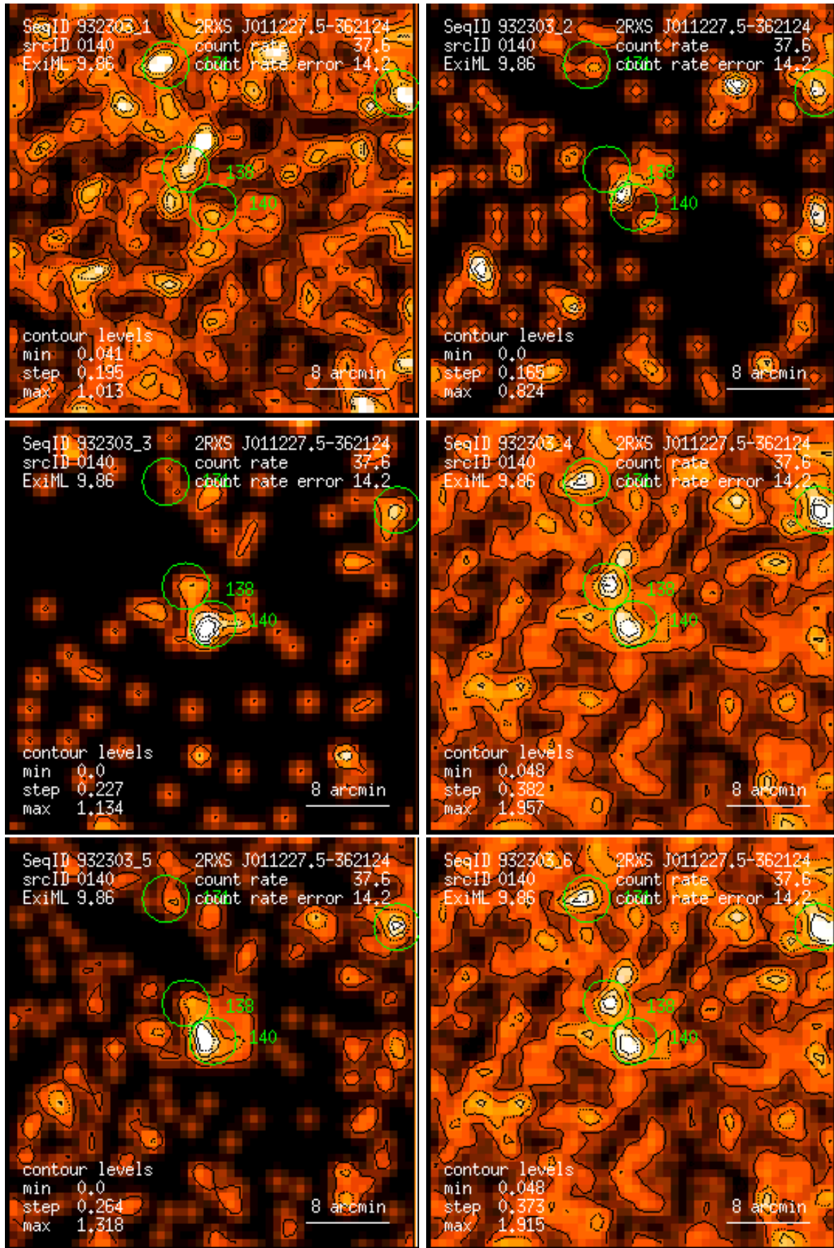
Figure 140: RASS 932303: detection 0140: band rate images, Gaussian filter: (1) PSPC channels 11 – 41, (2) 52 – 90, (3) 91 – 201, (4) 11 – 235, (5) 52 – 201, (6) 11 – 201. Broad band rates in counts/ks. Band rate contour levels in counts/ks/arcmin 2 .
