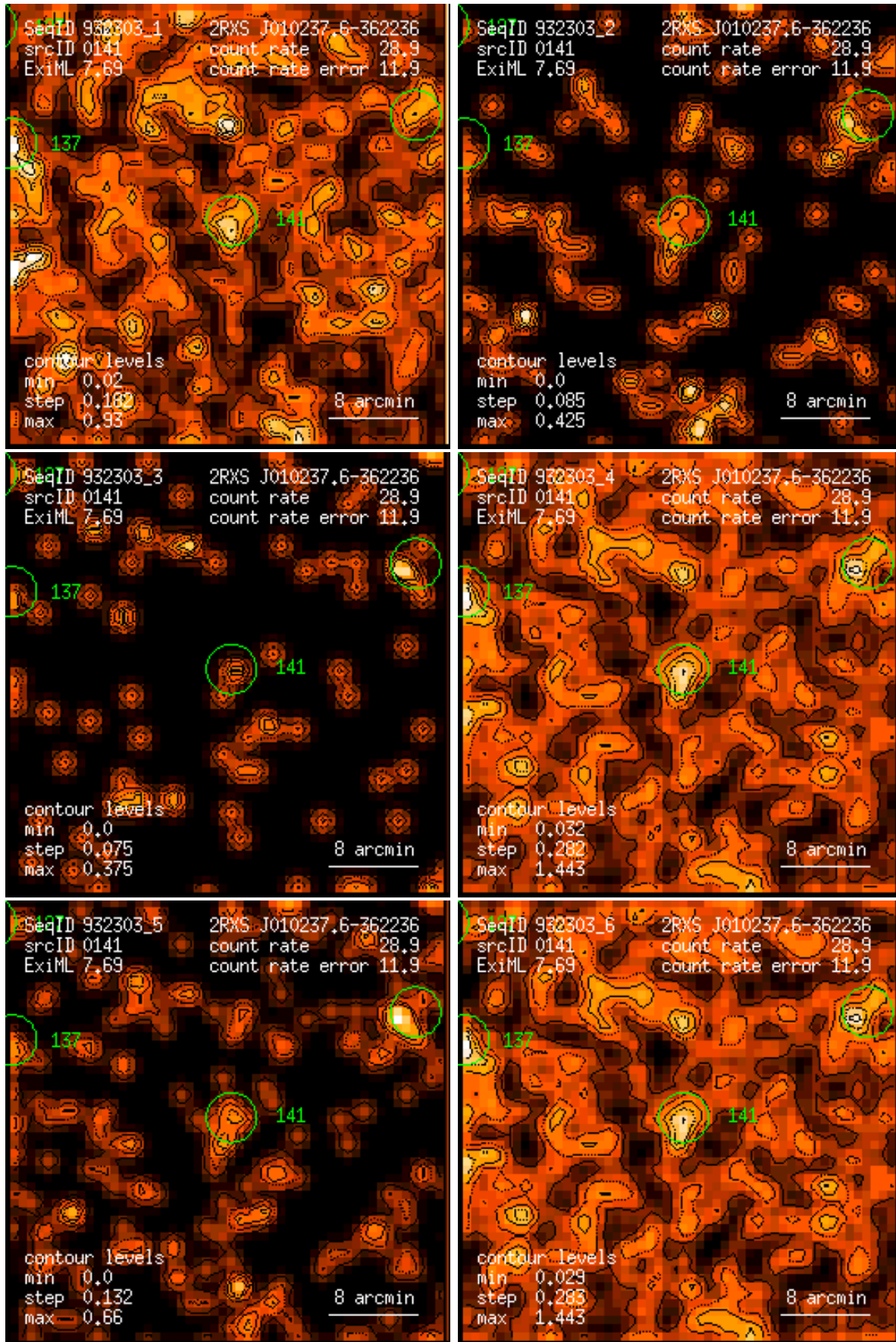
Figure 141: RASS 932303: detection 0141: band rate images, Gaussian filter: (1) PSPC channels 11 – 41, (2) 52 – 90, (3) 91 – 201, (4) 11 – 235, (5) 52 – 201, (6) 11 – 201. Broad band rates in counts/ks. Band rate contour levels in counts/ks/arcmin 2 .
