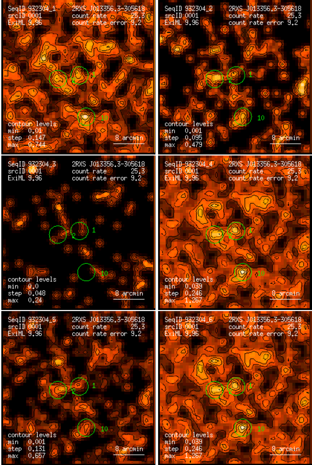
Figure 1: RASS 932304: detection 0001: band rate images, Gaussian filter: (1) PSPC channels 11 – 41, (2) 52 – 90, (3) 91 – 201, (4) 11 – 235, (5) 52 – 201, (6) 11 – 201. Broad band rates in counts/ks. Band rate contour levels in counts/ks/arcmin 2 .
