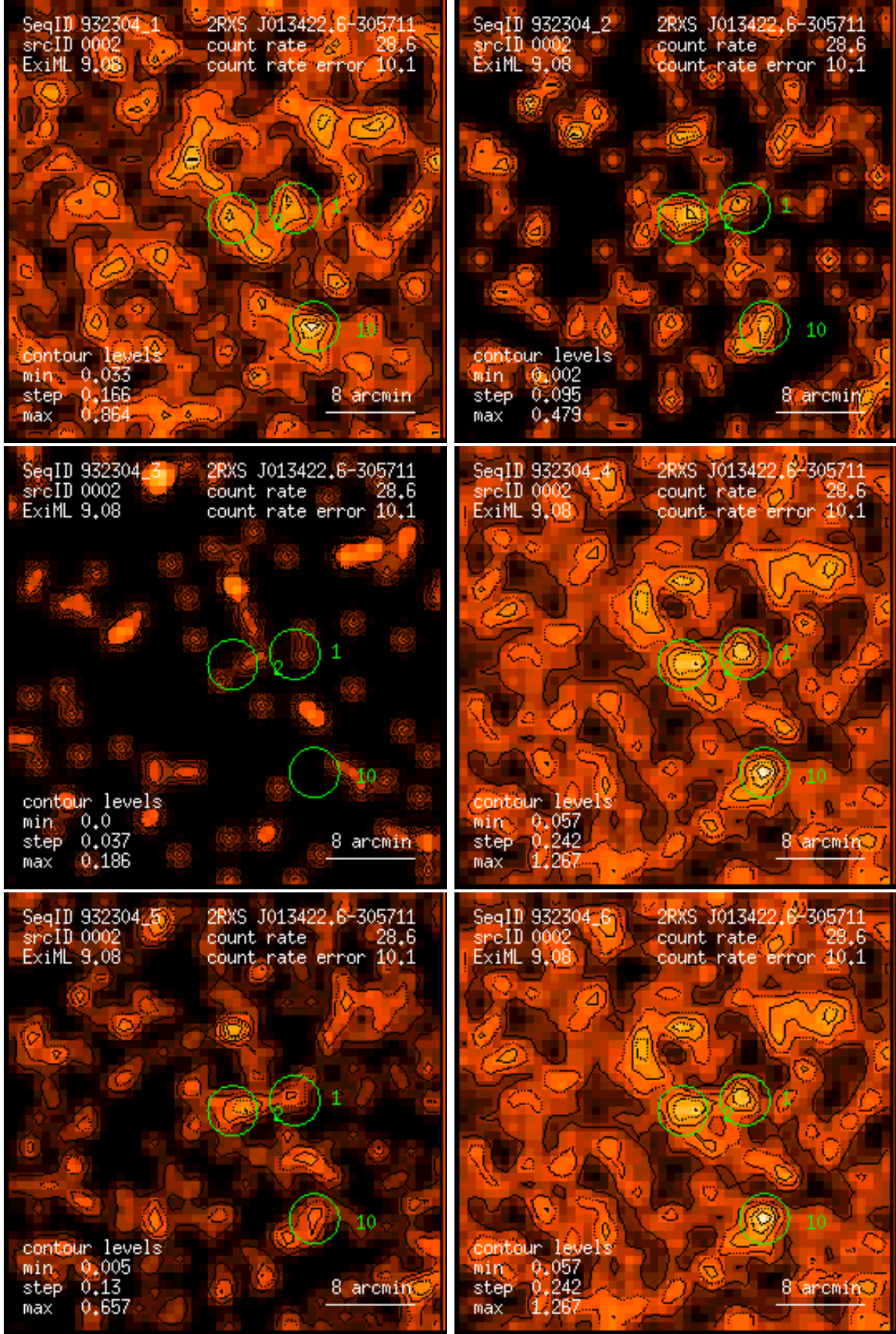
Figure 2: RASS 932304: detection 0002: band rate images, Gaussian filter: (1) PSPC channels 11 – 41, (2) 52 – 90, (3) 91 – 201, (4) 11 – 235, (5) 52 – 201, (6) 11 – 201. Broad band rates in counts/ks. Band rate contour levels in counts/ks/arcmin 2 .
