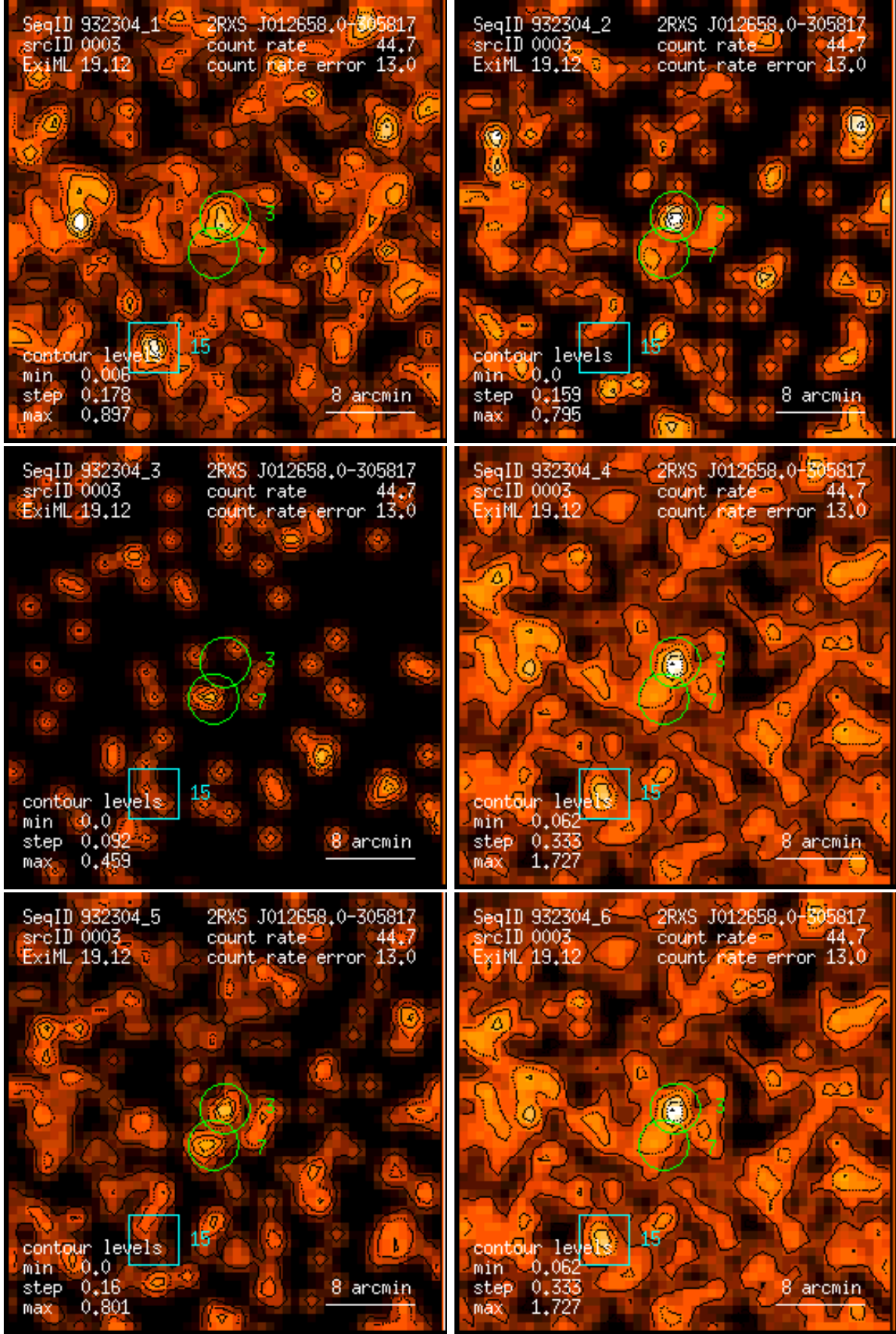
Figure 3: RASS 932304: detection 0003: band rate images, Gaussian filter: (1) PSPC channels 11 – 41, (2) 52 – 90, (3) 91 – 201, (4) 11 – 235, (5) 52 – 201, (6) 11 – 201. Broad band rates in counts/ks. Band rate contour levels in counts/ks/arcmin 2 .
