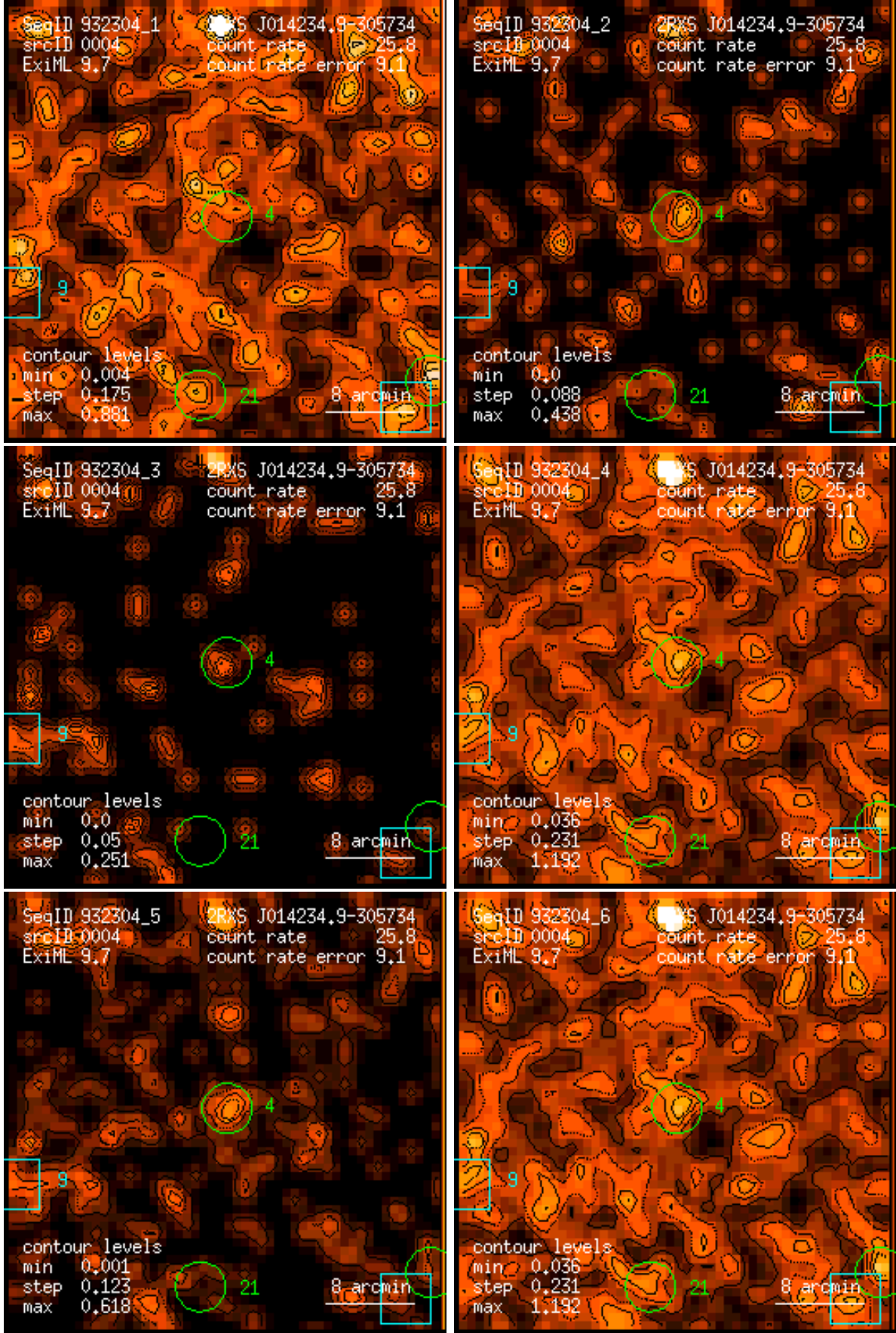
Figure 4: RASS 932304: detection 0004: band rate images, Gaussian filter: (1) PSPC channels 11 – 41, (2) 52 – 90, (3) 91 – 201, (4) 11 – 235, (5) 52 – 201, (6) 11 – 201. Broad band rates in counts/ks. Band rate contour levels in counts/ks/arcmin 2 .
