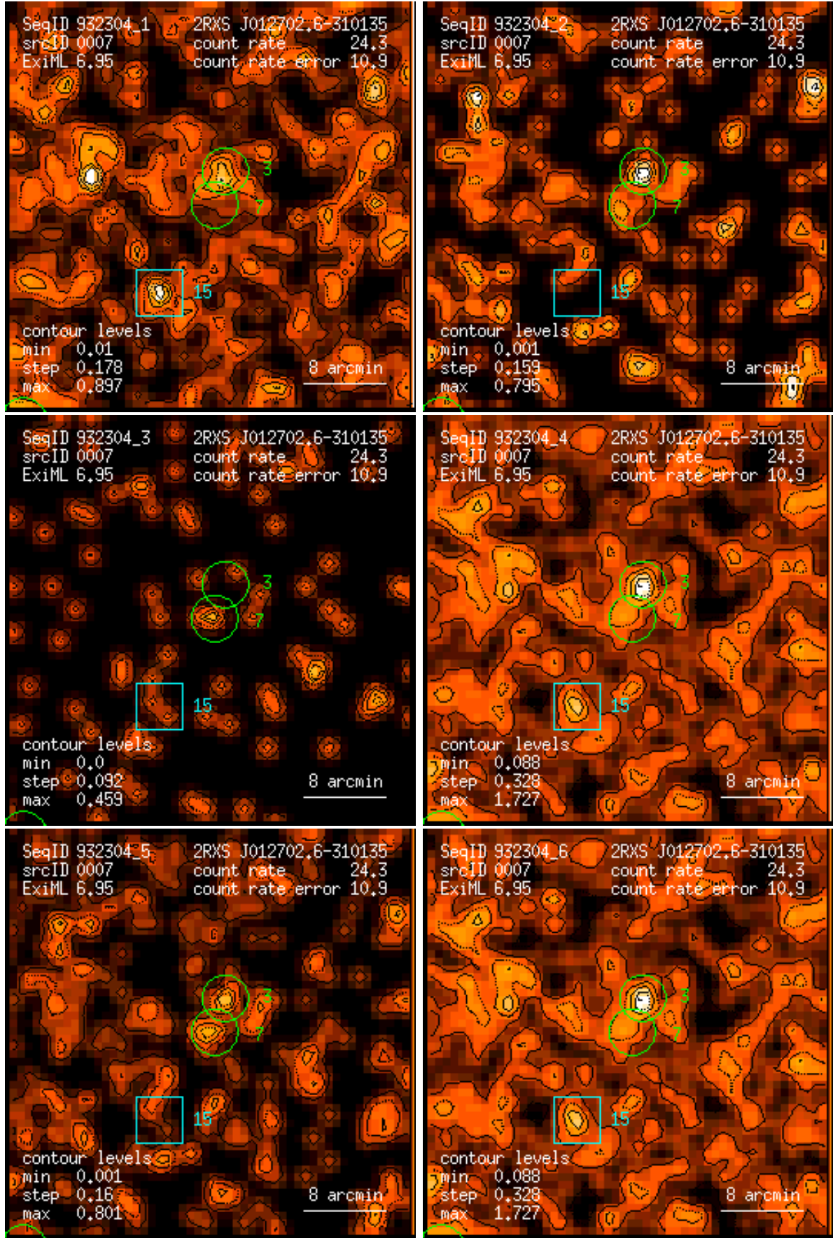
Figure 7: RASS 932304: detection 0007: band rate images, Gaussian filter: (1) PSPC channels 11 – 41, (2) 52 – 90, (3) 91 – 201, (4) 11 – 235, (5) 52 – 201, (6) 11 – 201. Broad band rates in counts/ks. Band rate contour levels in counts/ks/arcmin 2 .
