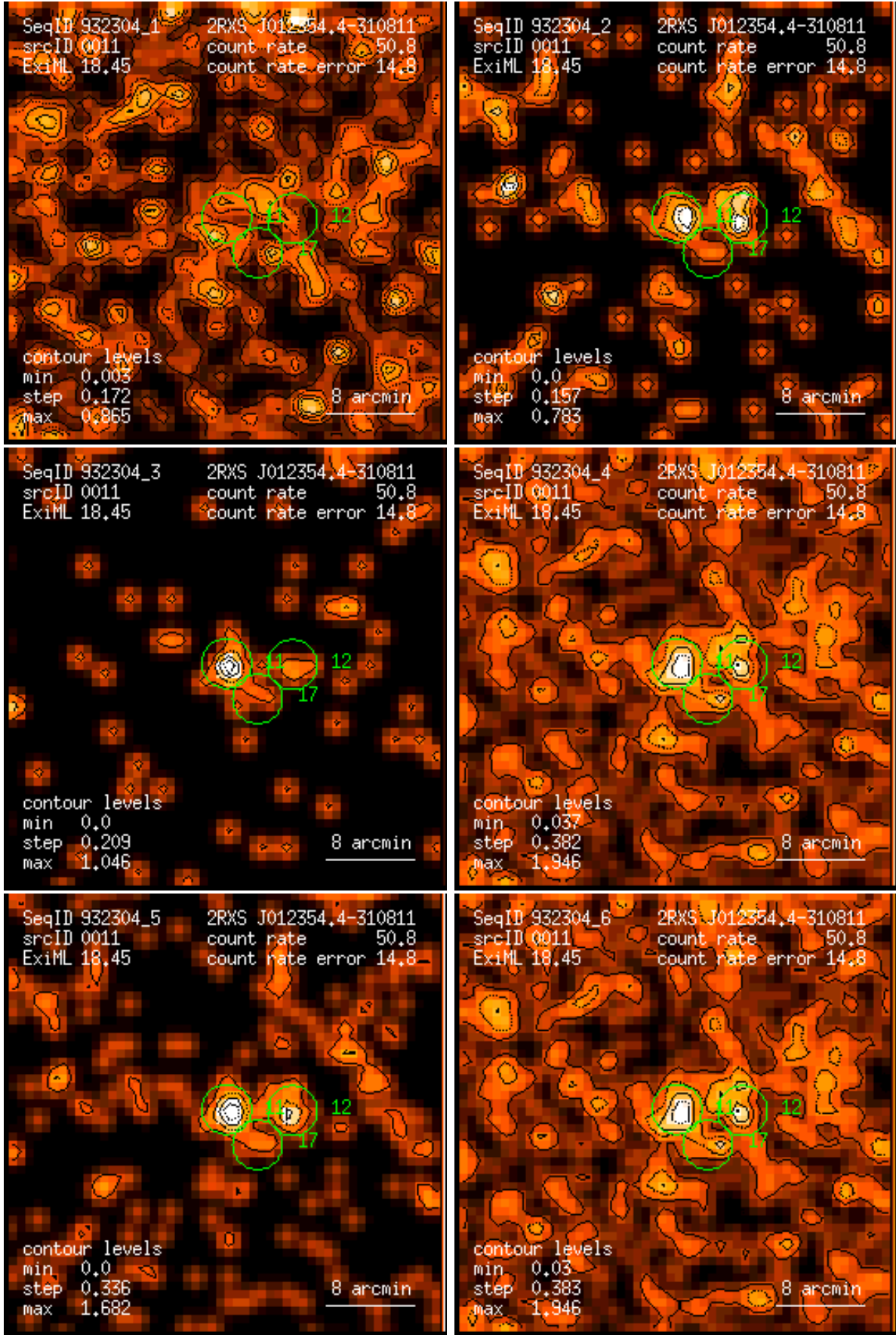
Figure 11: RASS 932304: detection 0011: band rate images, Gaussian filter: (1) PSPC channels 11 – 41, (2) 52 – 90, (3) 91 – 201, (4) 11 – 235, (5) 52 – 201, (6) 11 – 201. Broad band rates in counts/ks. Band rate contour levels in counts/ks/arcmin 2 .
