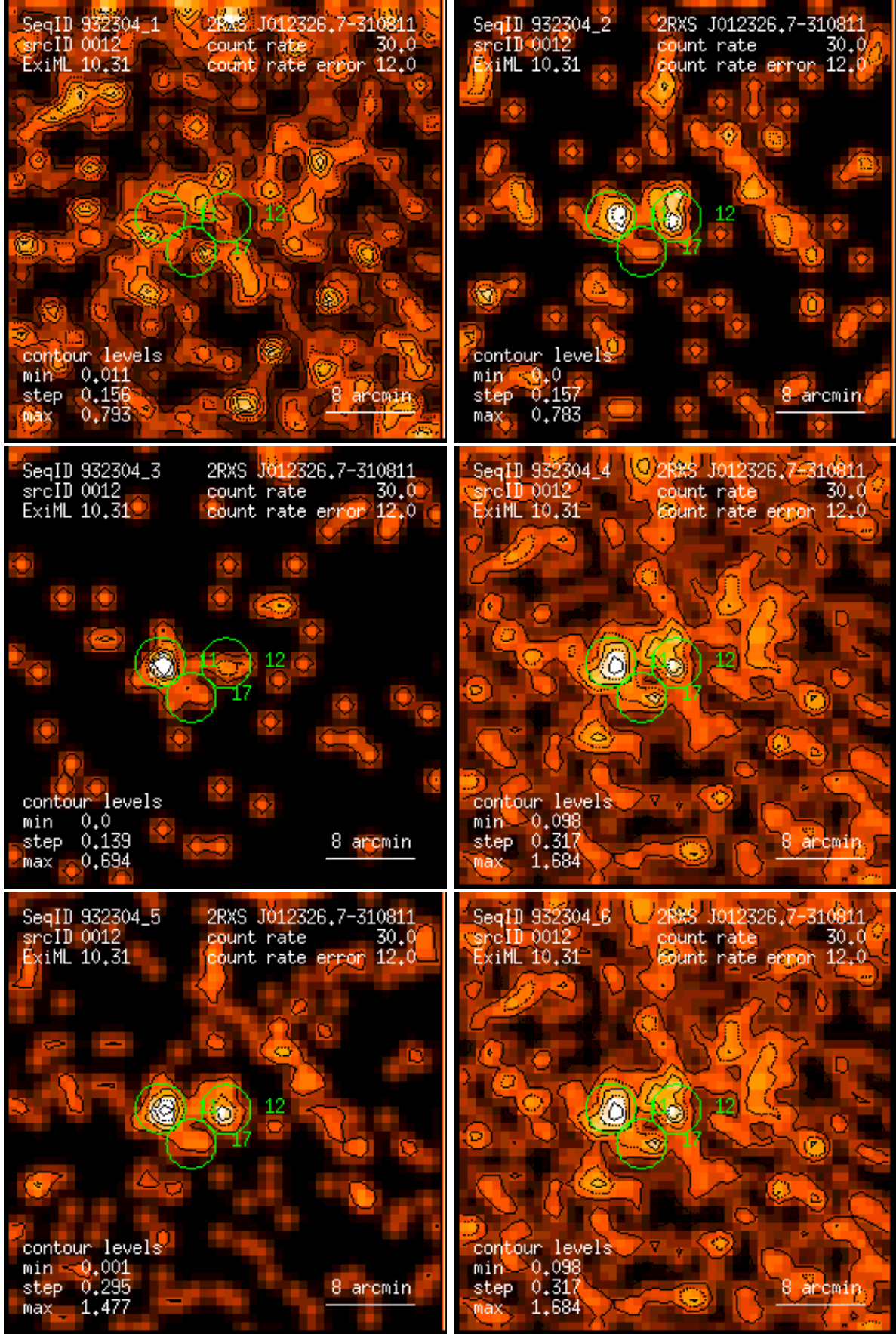
Figure 12: RASS 932304: detection 0012: band rate images, Gaussian filter: (1) PSPC channels 11 – 41, (2) 52 – 90, (3) 91 – 201, (4) 11 – 235, (5) 52 – 201, (6) 11 – 201. Broad band rates in counts/ks. Band rate contour levels in counts/ks/arcmin 2 .
