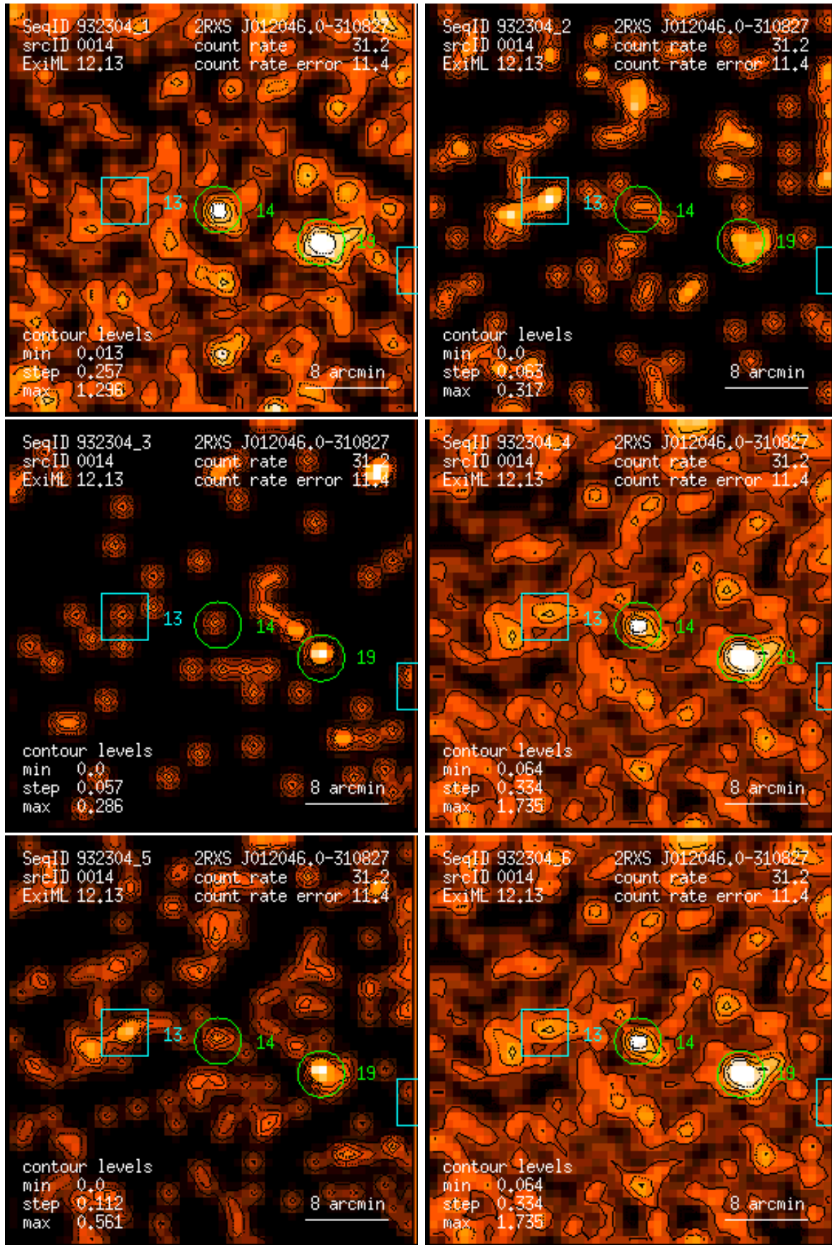
Figure 14: RASS 932304: detection 0014: band rate images, Gaussian filter: (1) PSPC channels 11 – 41, (2) 52 – 90, (3) 91 – 201, (4) 11 – 235, (5) 52 – 201, (6) 11 – 201. Broad band rates in counts/ks. Band rate contour levels in counts/ks/arcmin 2 .
