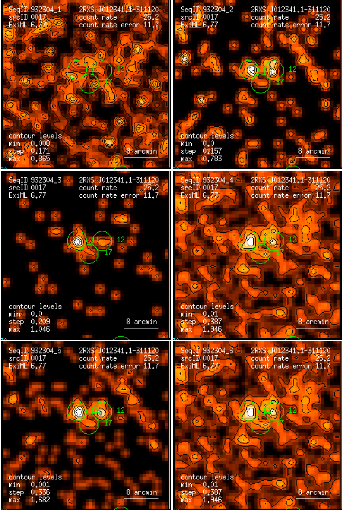
Figure 17: RASS 932304: detection 0017: band rate images, Gaussian filter: (1) PSPC channels 11 – 41, (2) 52 – 90, (3) 91 – 201, (4) 11 – 235, (5) 52 – 201, (6) 11 – 201. Broad band rates in counts/ks. Band rate contour levels in counts/ks/arcmin 2 .
