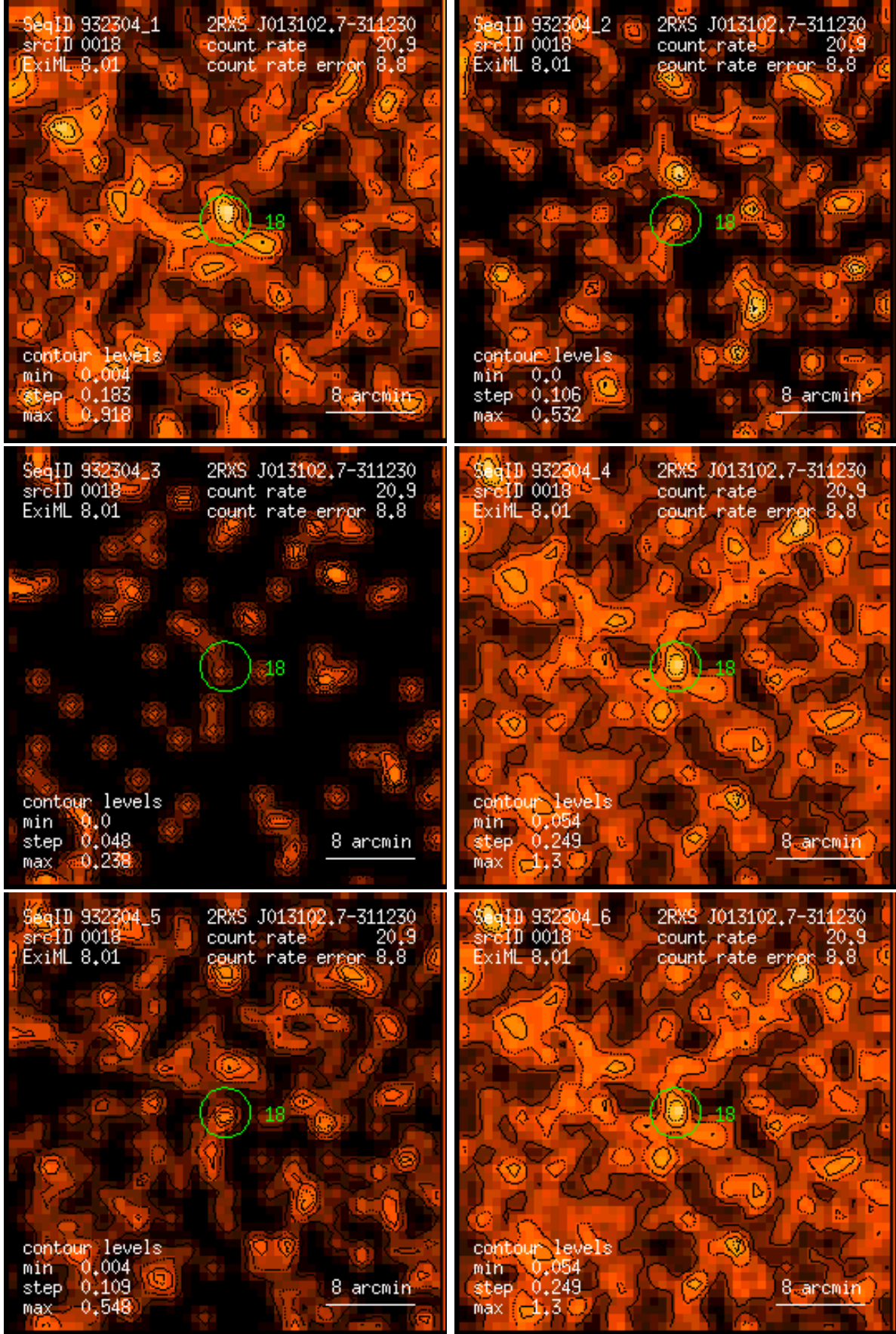
Figure 18: RASS 932304: detection 0018: band rate images, Gaussian filter: (1) PSPC channels 11 – 41, (2) 52 – 90, (3) 91 – 201, (4) 11 – 235, (5) 52 – 201, (6) 11 – 201. Broad band rates in counts/ks. Band rate contour levels in counts/ks/arcmin 2 .
