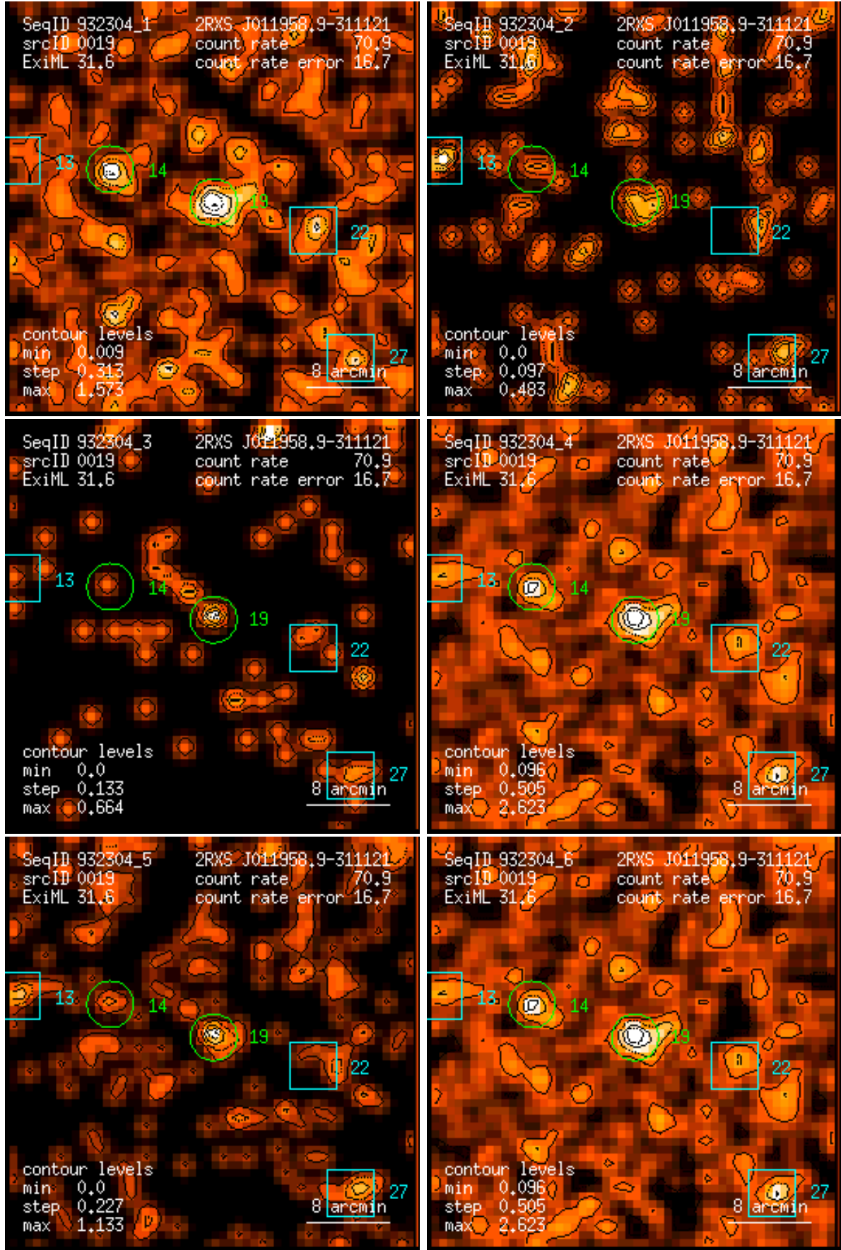
Figure 19: RASS 932304: detection 0019: band rate images, Gaussian filter: (1) PSPC channels 11 – 41, (2) 52 – 90, (3) 91 – 201, (4) 11 – 235, (5) 52 – 201, (6) 11 – 201. Broad band rates in counts/ks. Band rate contour levels in counts/ks/arcmin 2 .
