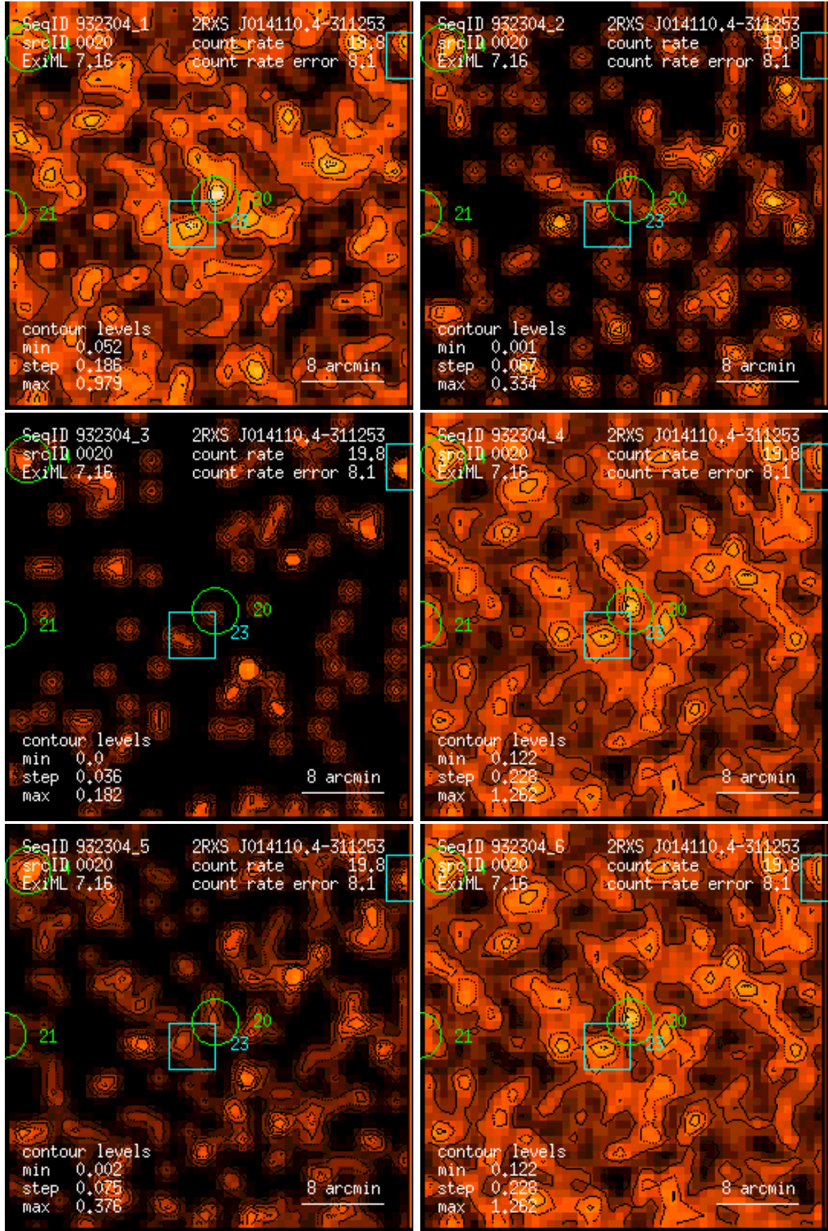
Figure 20: RASS 932304: detection 0020: band rate images, Gaussian filter: (1) PSPC channels 11 – 41, (2) 52 – 90, (3) 91 – 201, (4) 11 – 235, (5) 52 – 201, (6) 11 – 201. Broad band rates in counts/ks. Band rate contour levels in counts/ks/arcmin 2 .
