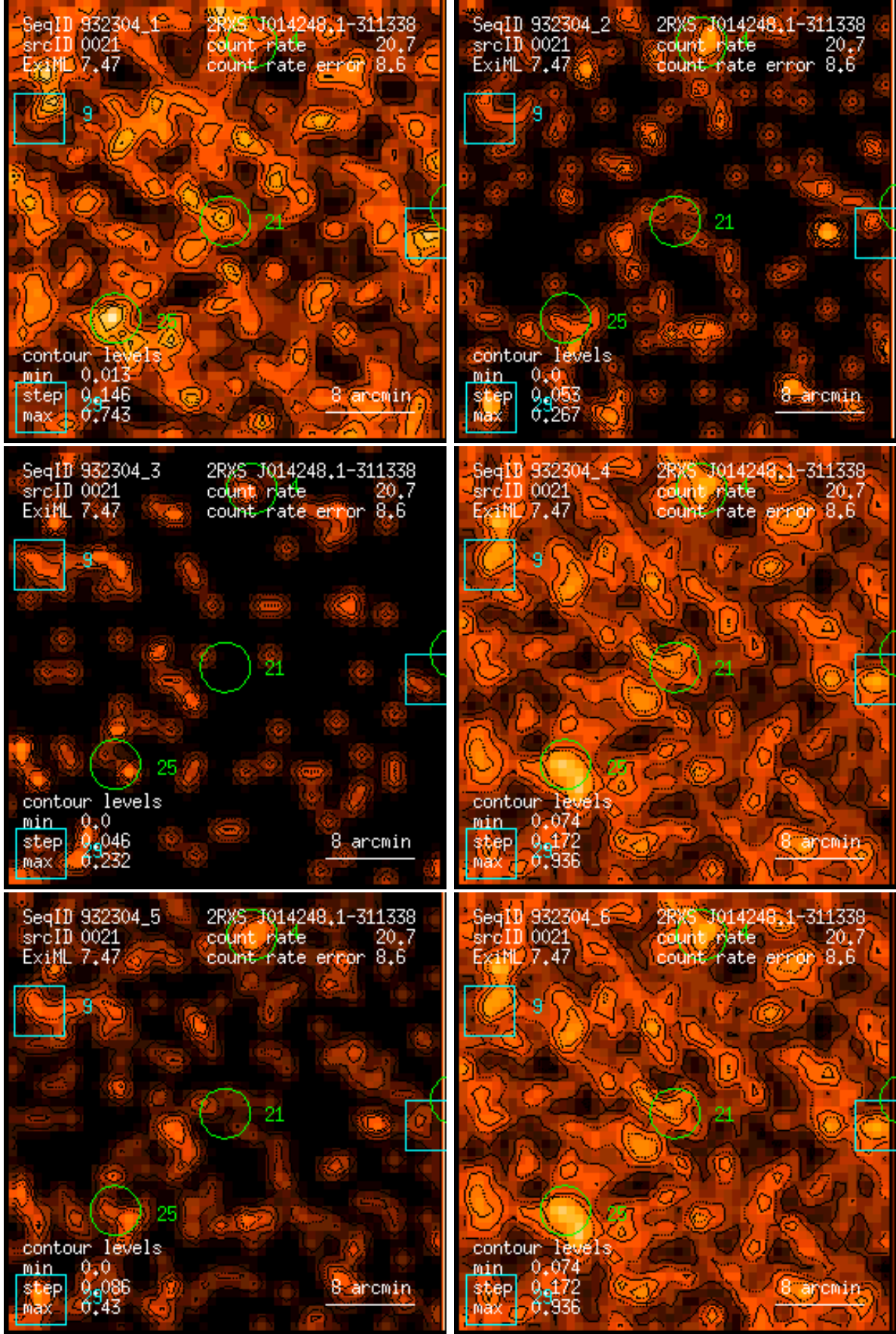
Figure 21: RASS 932304: detection 0021: band rate images, Gaussian filter: (1) PSPC channels 11 – 41, (2) 52 – 90, (3) 91 – 201, (4) 11 – 235, (5) 52 – 201, (6) 11 – 201. Broad band rates in counts/ks. Band rate contour levels in counts/ks/arcmin 2 .
