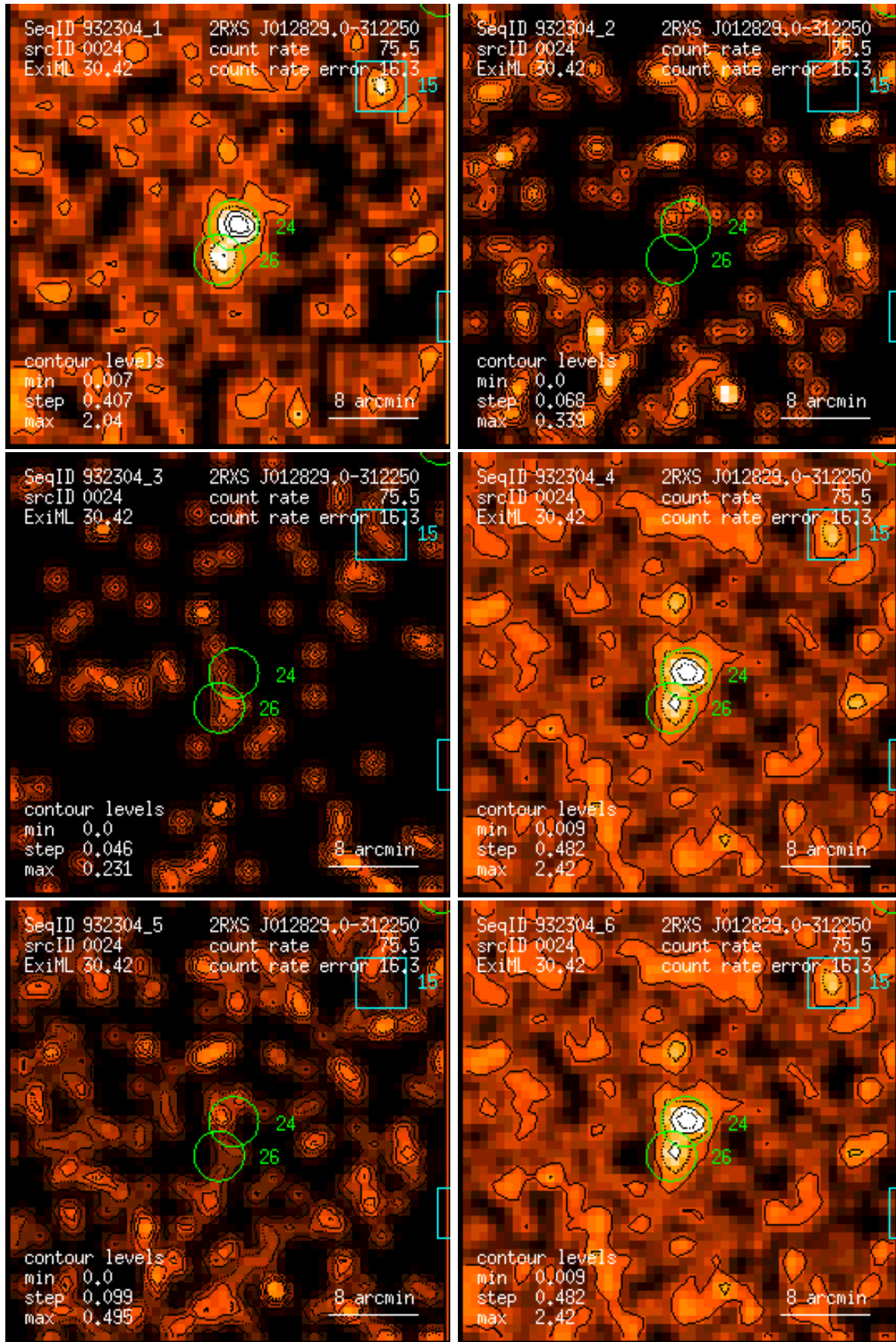
Figure 24: RASS 932304: detection 0024: band rate images, Gaussian filter: (1) PSPC channels 11 – 41, (2) 52 – 90, (3) 91 – 201, (4) 11 – 235, (5) 52 – 201, (6) 11 – 201. Broad band rates in counts/ks. Band rate contour levels in counts/ks/arcmin 2 .
