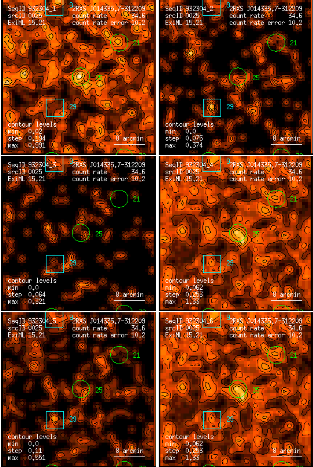
Figure 25: RASS 932304: detection 0025: band rate images, Gaussian filter: (1) PSPC channels 11 – 41, (2) 52 – 90, (3) 91 – 201, (4) 11 – 235, (5) 52 – 201, (6) 11 – 201. Broad band rates in counts/ks. Band rate contour levels in counts/ks/arcmin 2 .
