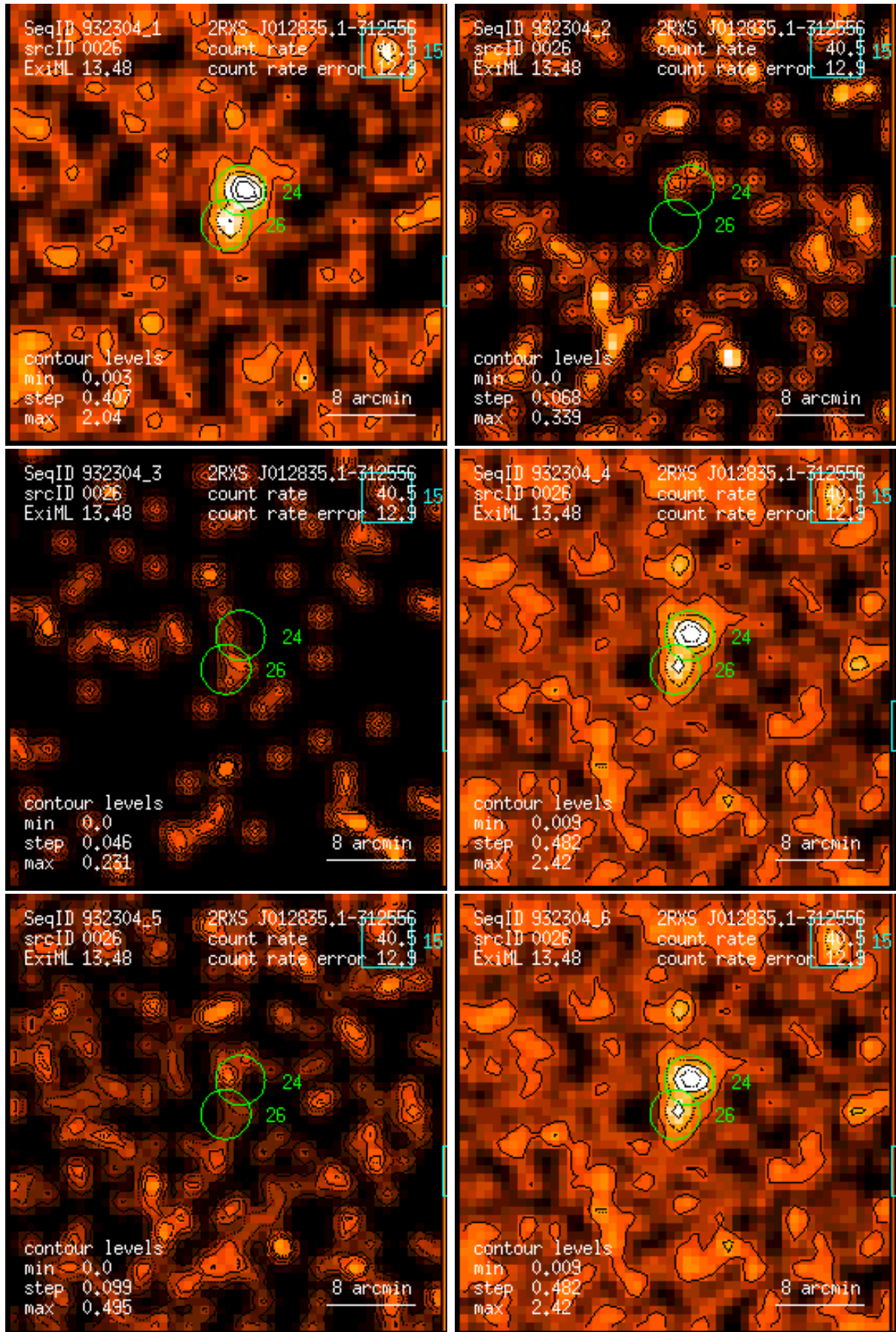
Figure 26: RASS 932304: detection 0026: band rate images, Gaussian filter: (1) PSPC channels 11 – 41, (2) 52 – 90, (3) 91 – 201, (4) 11 – 235, (5) 52 – 201, (6) 11 – 201. Broad band rates in counts/ks. Band rate contour levels in counts/ks/arcmin 2 .
