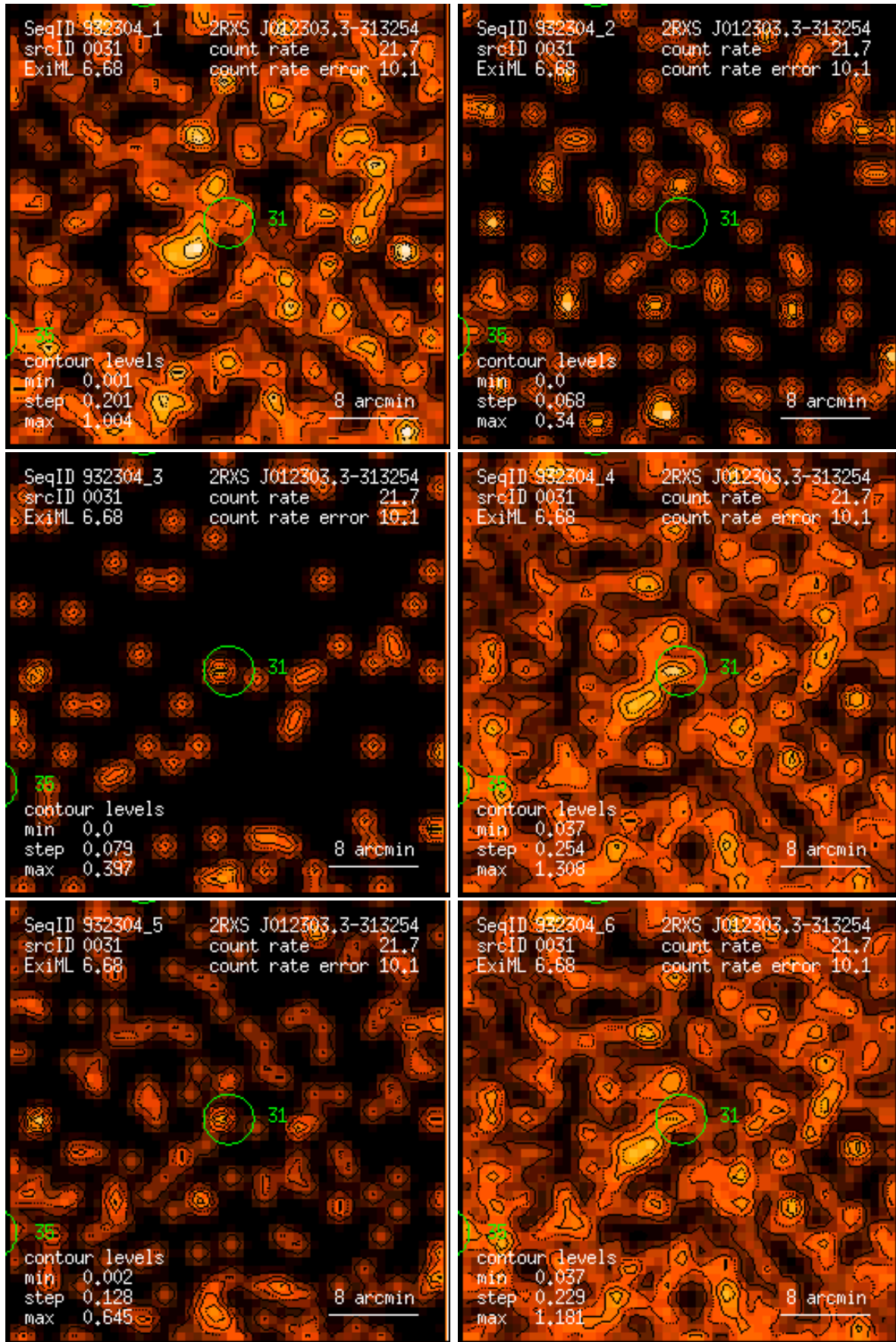
Figure 31: RASS 932304: detection 0031: band rate images, Gaussian filter: (1) PSPC channels 11 – 41, (2) 52 – 90, (3) 91 – 201, (4) 11 – 235, (5) 52 – 201, (6) 11 – 201. Broad band rates in counts/ks. Band rate contour levels in counts/ks/arcmin 2 .
