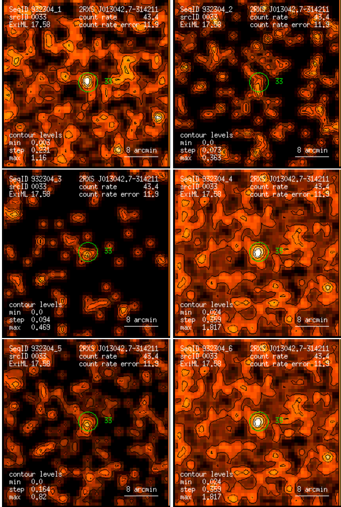
Figure 33: RASS 932304: detection 0033: band rate images, Gaussian filter: (1) PSPC channels 11 – 41, (2) 52 – 90, (3) 91 – 201, (4) 11 – 235, (5) 52 – 201, (6) 11 – 201. Broad band rates in counts/ks. Band rate contour levels in counts/ks/arcmin 2 .
